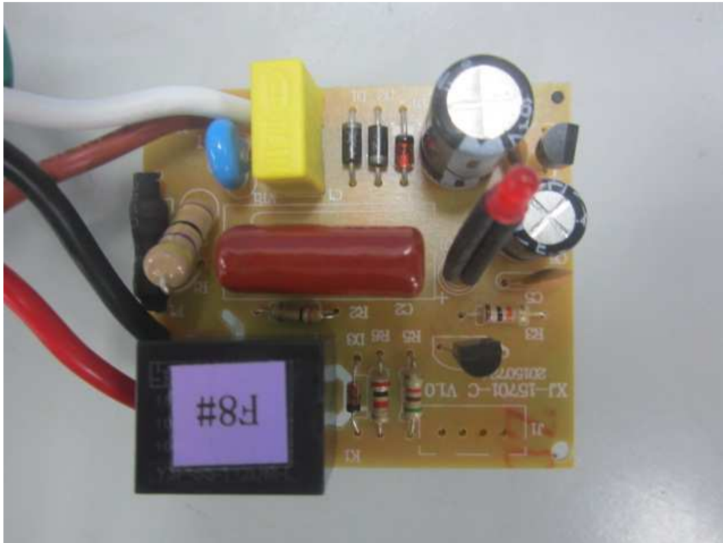
Main PCB view (Remove RF Module)
