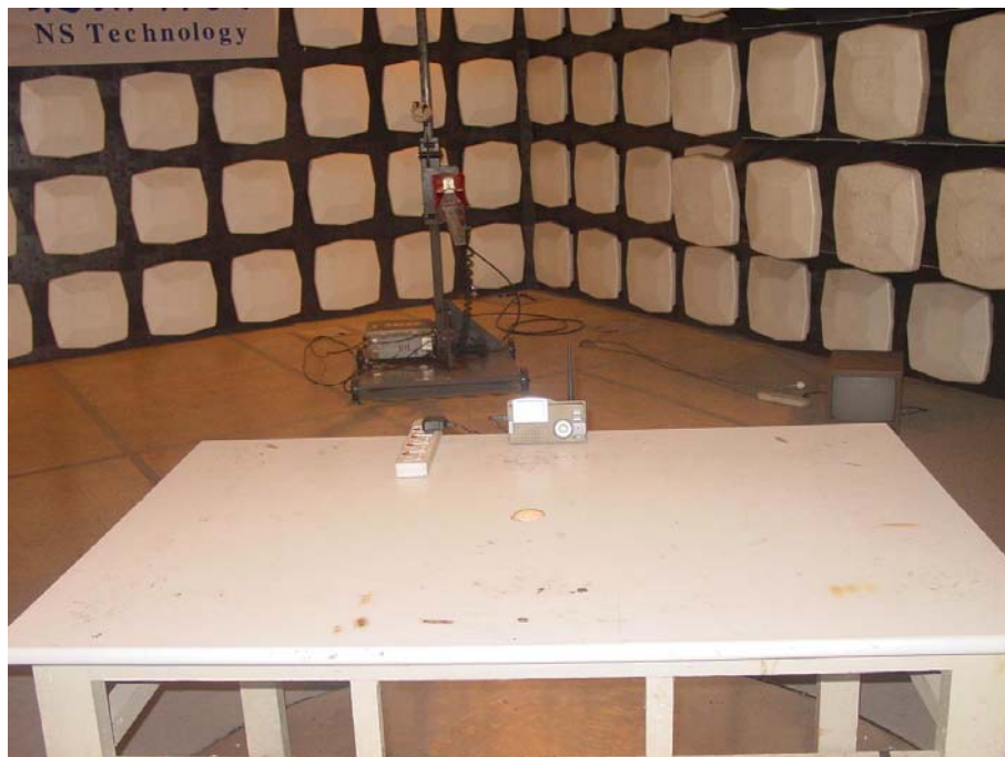
Figure 2 Test photo of Transmitter Spurious Emission (TX Mode above 1G)
