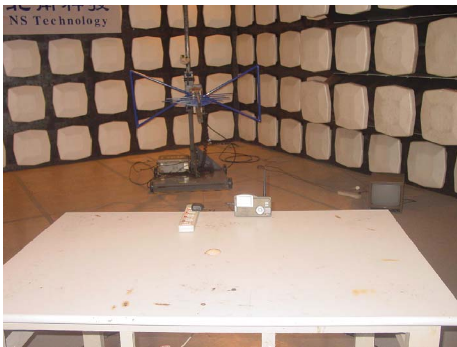
Figure 1 Test photo of Transmitter Spurious Emission (TX Mode 30-1000MHz)
