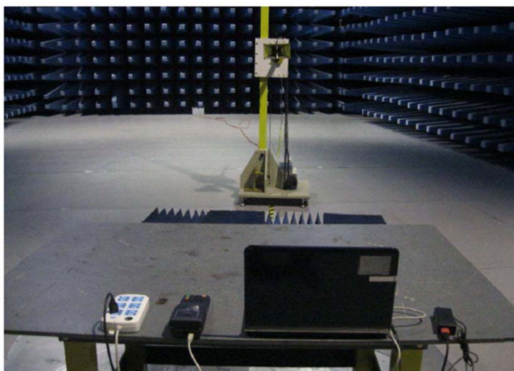
Radiated Emission Test Setup Front View Above 1GHz
