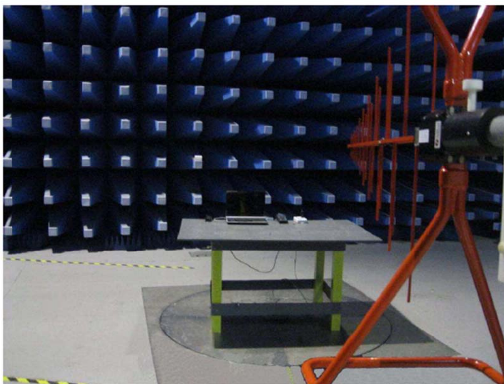
Radiated Emission Test Setup Front View Below 1GHz
