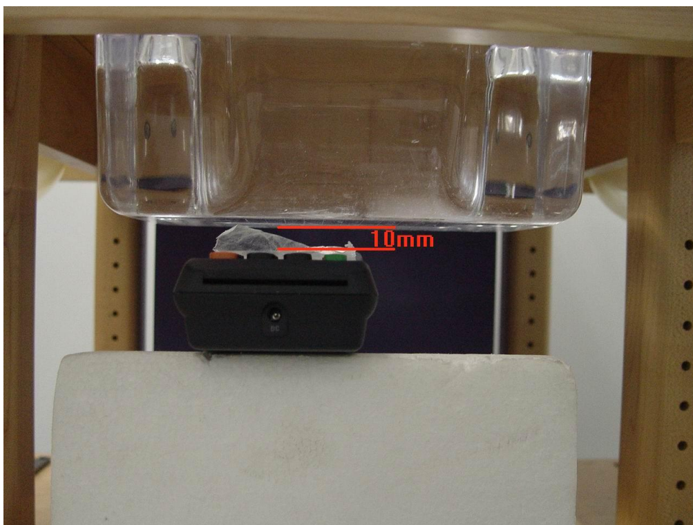
Figure B.2 EUT Front side Towards phantom
