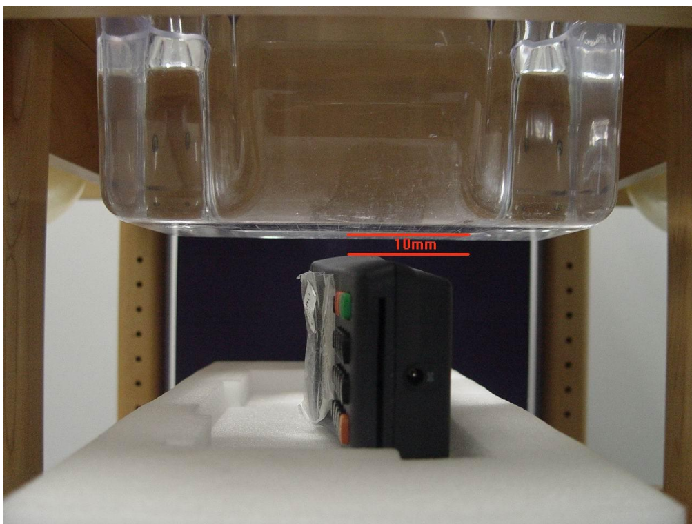
Figure B.5 EUT Right side Towards phantom
