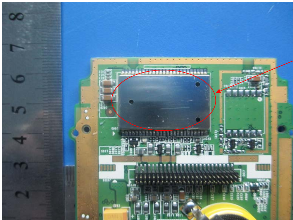
GPRS Antenna Module Front View
