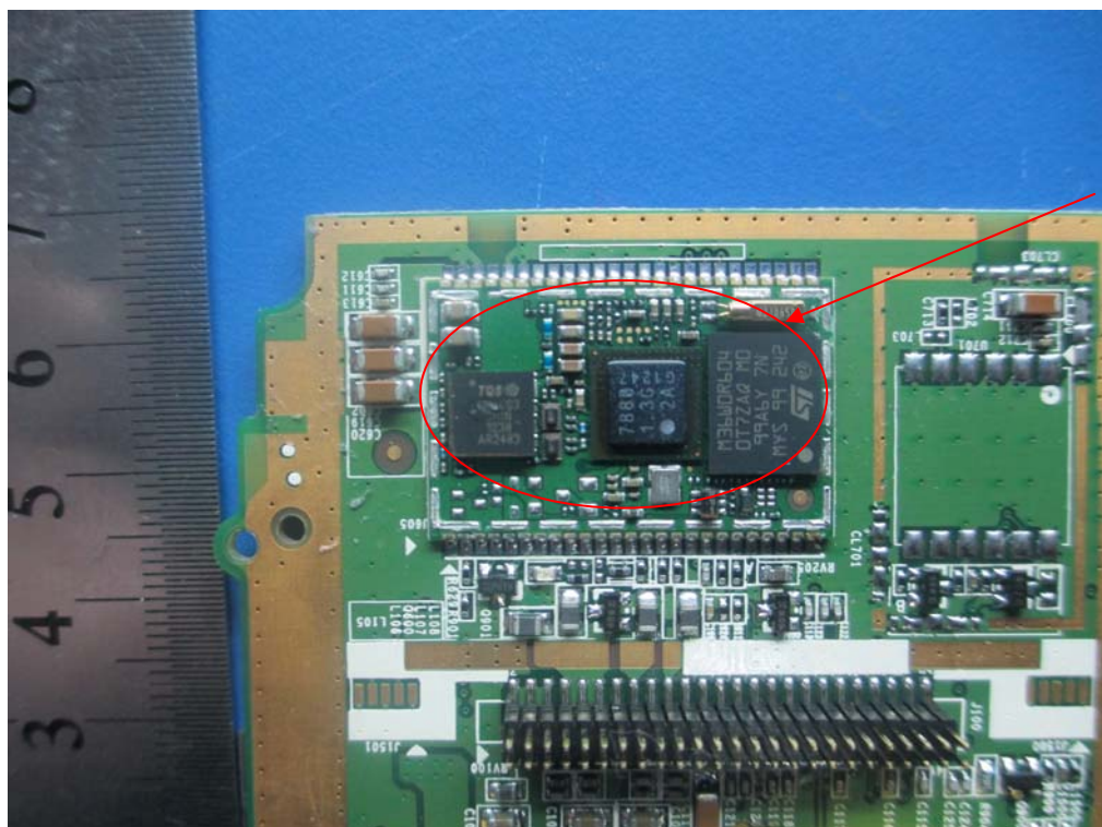
GPRS Antenna Module Shielding off Front View
