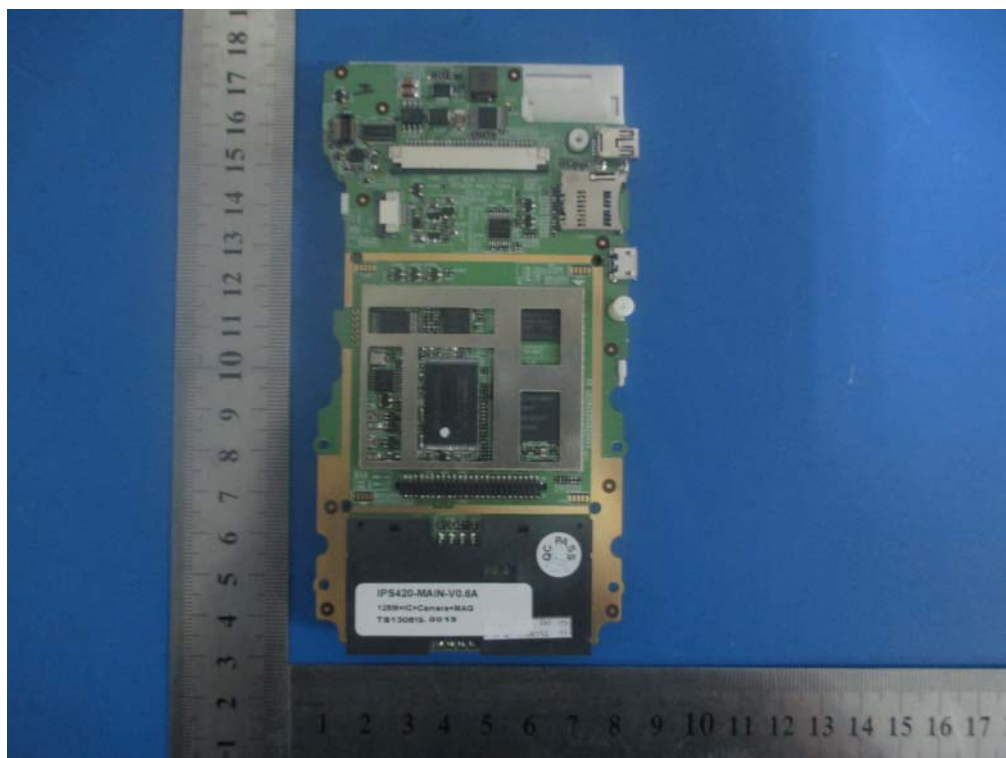
PCB 1 Shielding off - Bottom View
