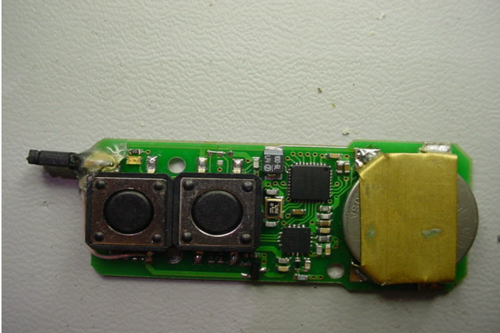
Internal RF board front view
