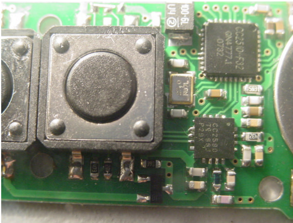
Internal RF board front view component information
