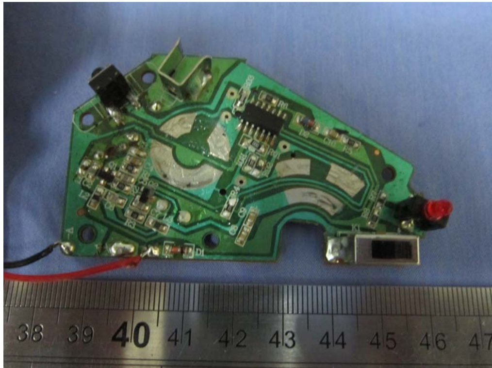
Rear View of PCB
