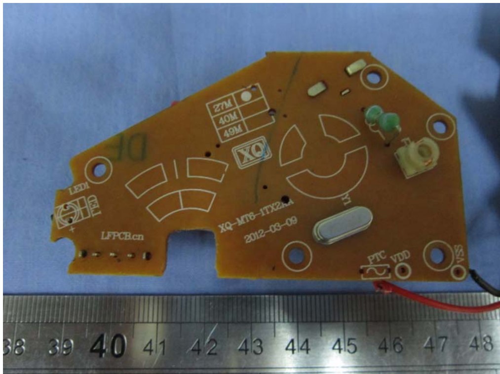
Front View of PCB
