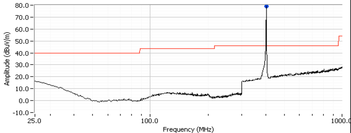
25 - 1000 MHz, Low Channel @ 402.45 MHz, EUT flat Orientation
