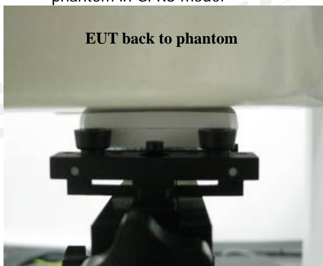
Fig.4 Testing body-worn SAR the back side of the EUT is paralleled and contact with flat phantom in GPRS mode.
