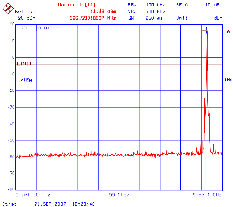
Plot 6.8.5.2.3(i) Spurious RF Conducted Emissions Transmitter Frequency: 926 MHz
