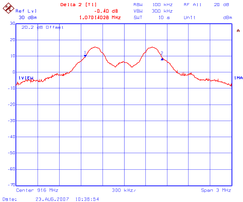
Plot 6.6.5.2 6 dB Bandwidth Frequency: 916 MHz
