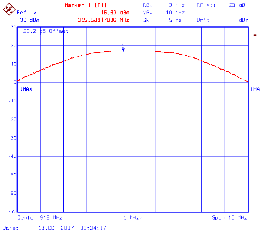
Plot 6.7.5.5 Peak Conducted Output Power Frequency: 916 MHz; Input Voltage: 3.6 VDC
