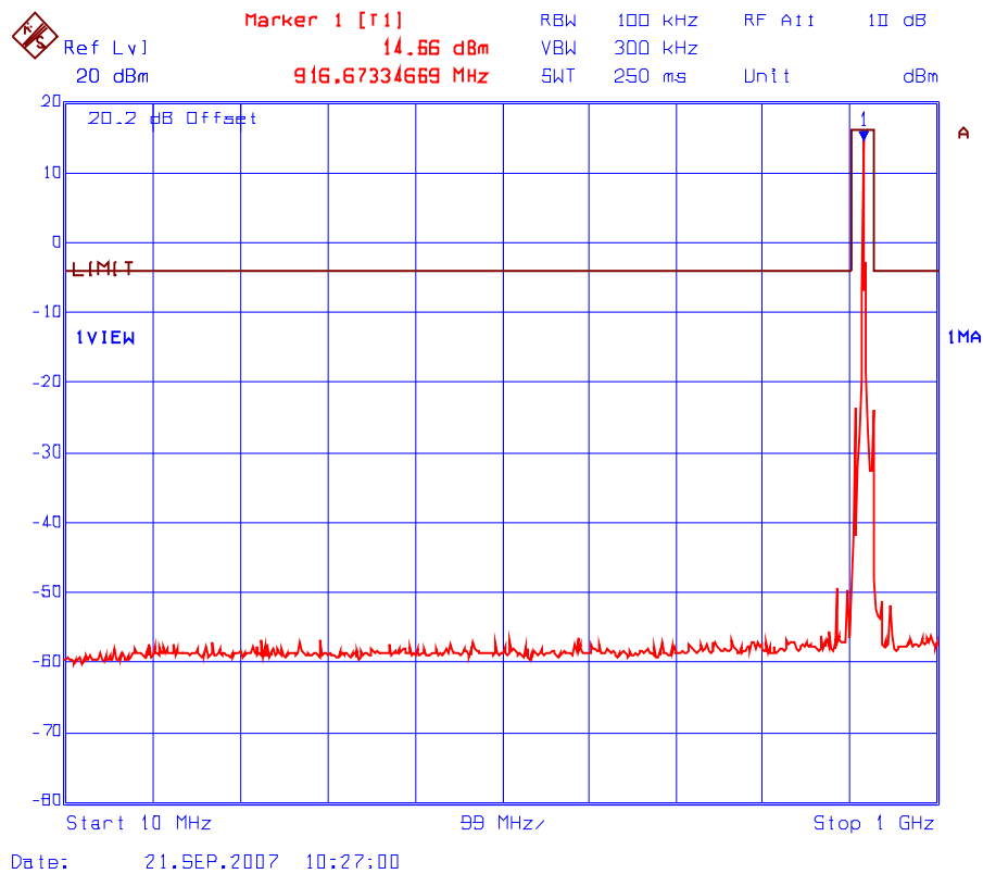
Plot 6.8.5.2(i) Spurious RF Conducted Emissions Transmitter Frequency: 916 MHz
