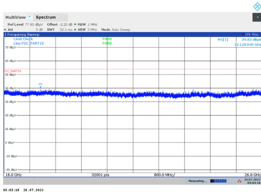
Plot 4: 18 GHz to 26 GHz, vertical & horizontal polarization, valid for all channels and all modes
