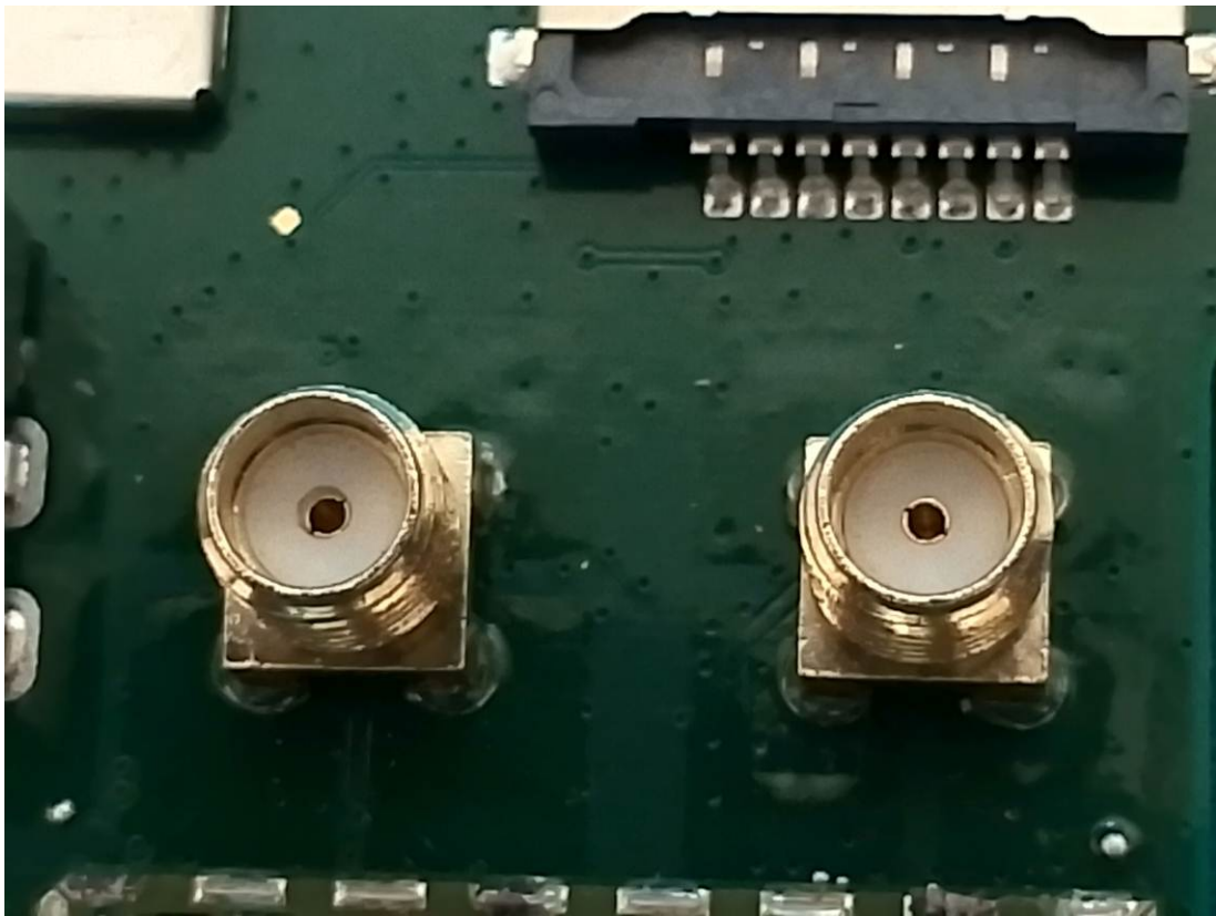
WWAN Antenna port
