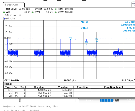
BLE_1M_Middle_Channel
