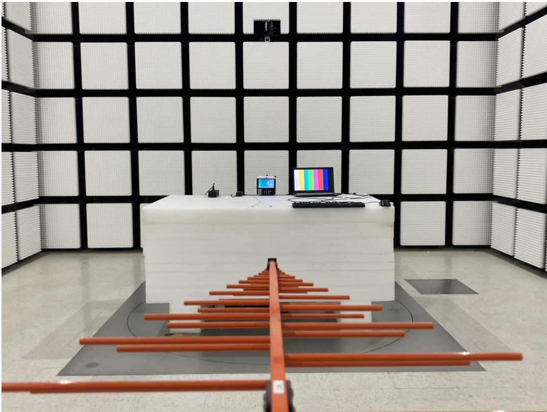
Radiated Emission Below 1GHz rear View Adapter 2# M5
