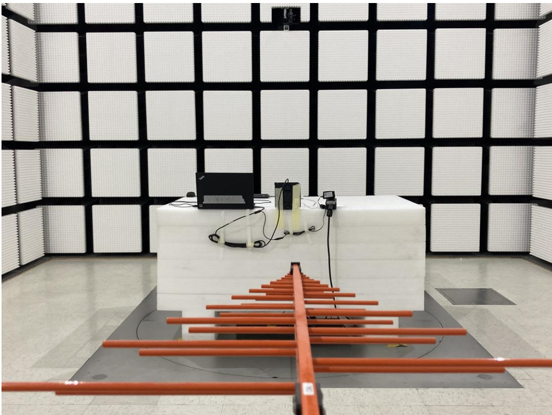
Radiated Emission Below 1GHz rear View M4
