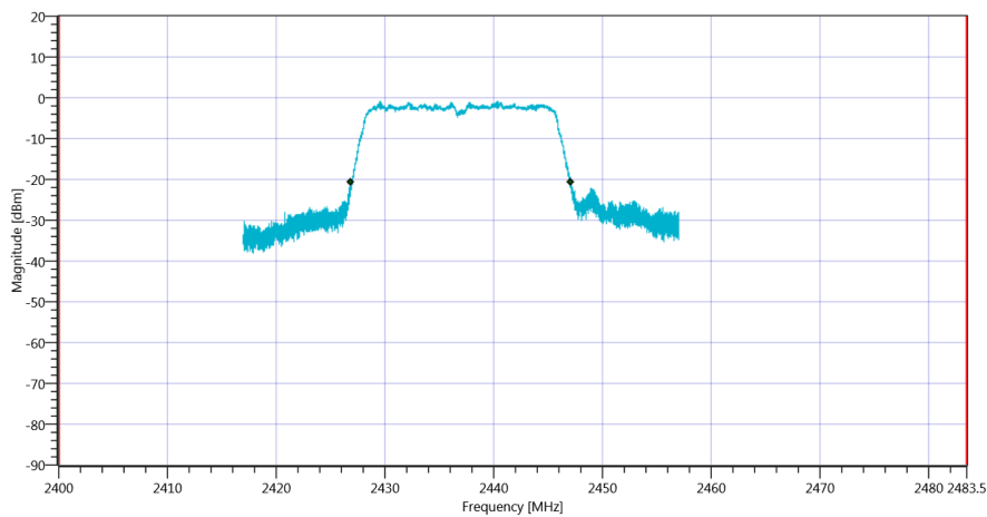
Plot_FCC Part 15.247 Bandwidth 99PCT-20dB ~ WLAN2G4 nHT20-mode_04072019_130751.png
