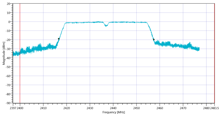
Plot_FCC Part 15.247 Bandwidth 99PCT-20dB ~ WLAN2G4 nHT40-mode_04072019_140307.png
