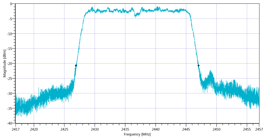
Plot_FCC Part 15.247 Bandwidth 99PCT-20dB ~ WLAN2G4 nHT20-mode_04072019_130748.png
