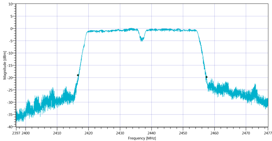
Plot_FCC Part 15.247 Bandwidth 99PCT-20dB ~ WLAN2G4 nHT40-mode 20dB_04072019_140304.png
