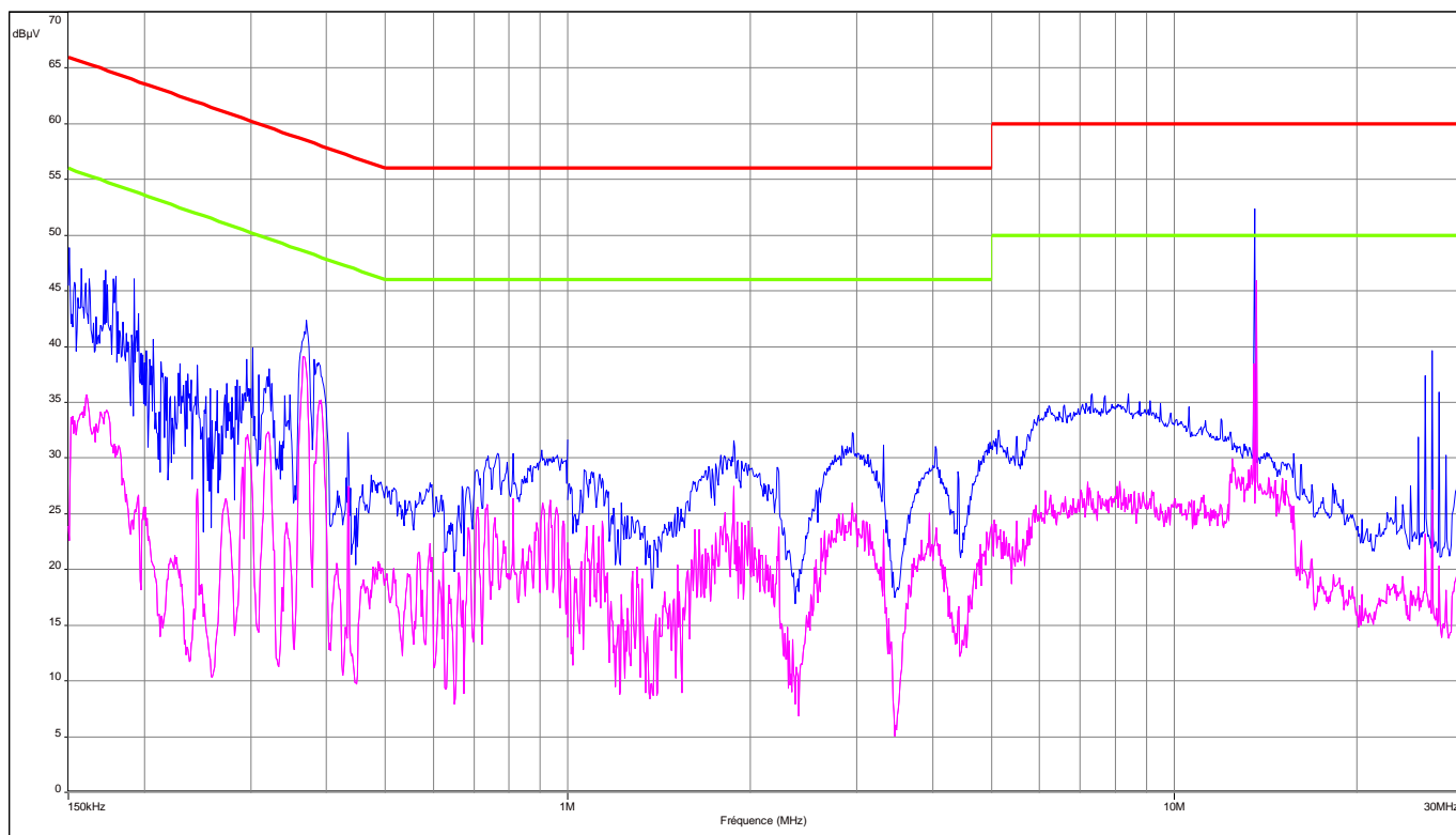
Diagram N°2 Neutral
