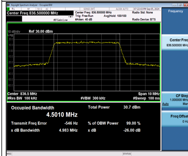
Band26(824-849)-5MHz-16QAM-26915-25RB#0-PASS
