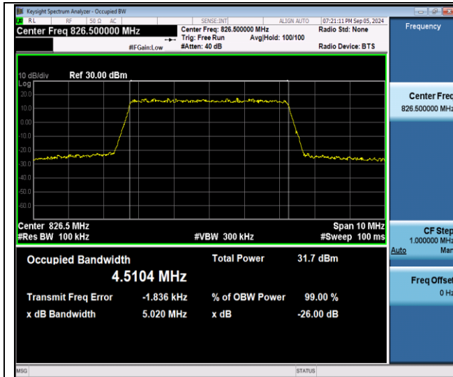
Band26(824-849)-5MHz-QPSK-26815-25RB#0-PASS
