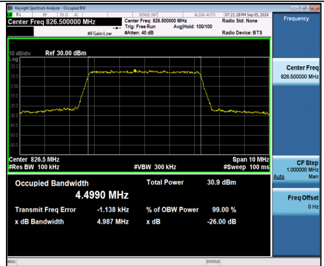
Band26(824-849)-5MHz-16QAM-26815-25RB#0-PASS
