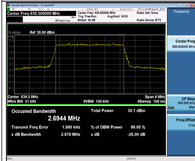
Band26(824-849)-3MHz-16QAM-26915-15RB#0-PASS
