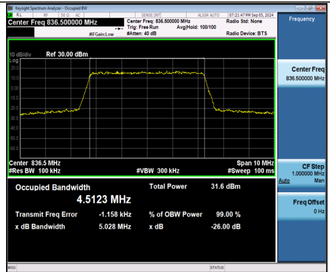
Band26(824-849)-5MHz-QPSK-26915-25RB#0-PASS
