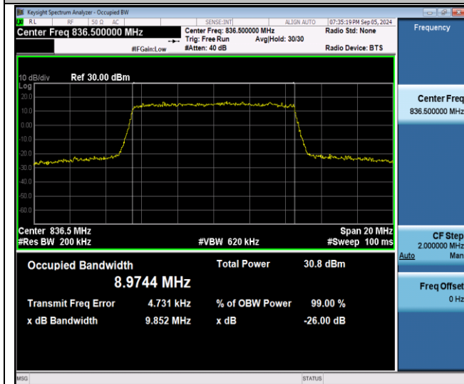
Band26(824-849)-10MHz-16QAM-26915-50RB#0-PASS
