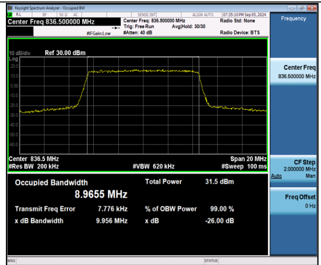
Band26(824-849)-10MHz-QPSK-26915-50RB#0-PASS
