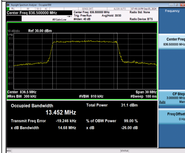
Band26(824-849)-15MHz-16QAM-26915-75RB#0-PASS
