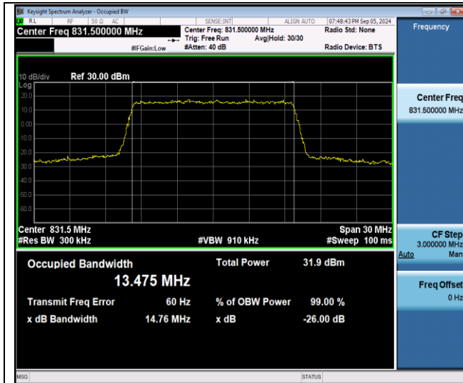
Band26(824-849)-15MHz-QPSK-26865-75RB#0-PASS
