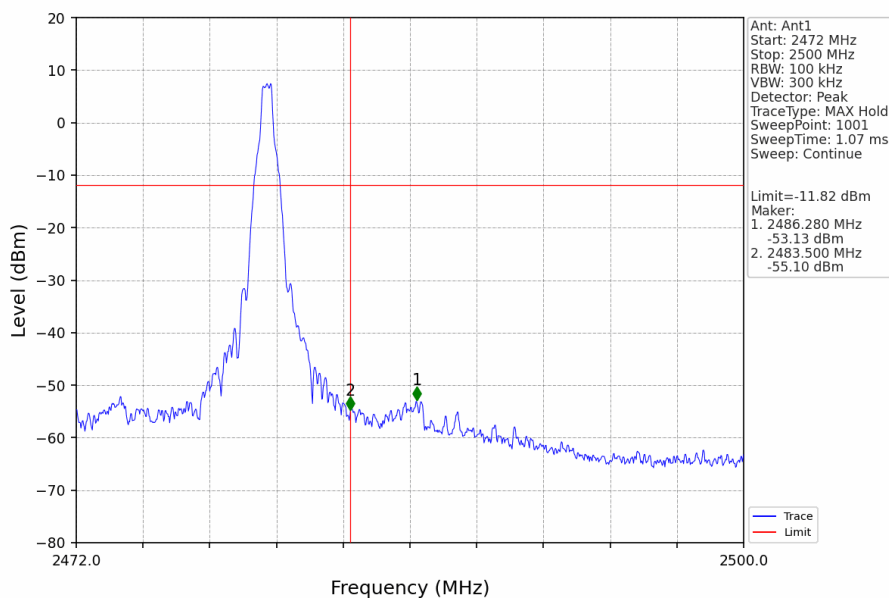
GFSK_DH5_HCH_2480MHz_Ant1_NTNV
