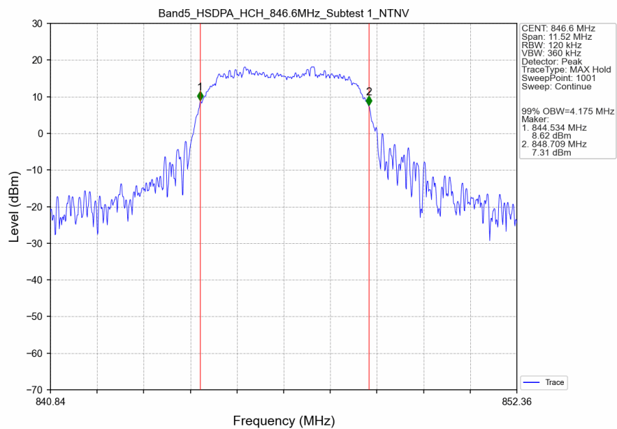
Band5_HSDPA_HCH_846.6MHz_Subtest 1_NTNV
