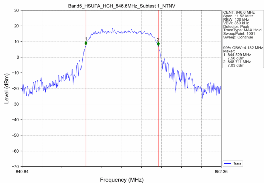
Band5_HSUPA_HCH_846.6MHz_Subtest 1_NTNV
