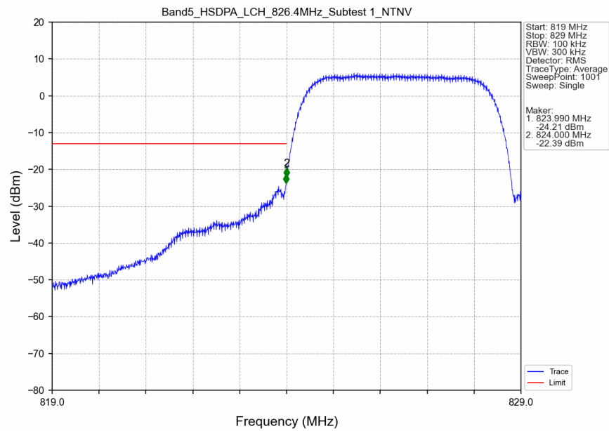
Band5_HSDPA_LCH_826.4MHz_Subtest 1_NTNV
