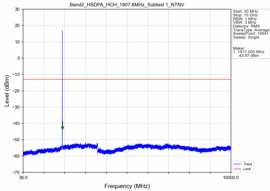
Band2_HSDPA_HCH_1907.6MHz_Subtest 1_NTNV
