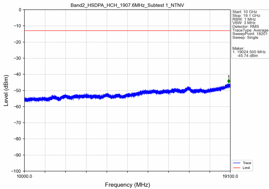
Band2_HSDPA_HCH_1907.6MHz_Subtest 1_NTNV
