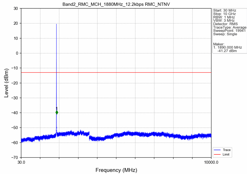
Band2_RMC_MCH_1880MHz_12.2kbps RMC_NTNV
