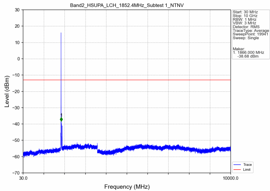
Band2_HSUPA_LCH_1852.4MHz_Subtest 1_NTNV
