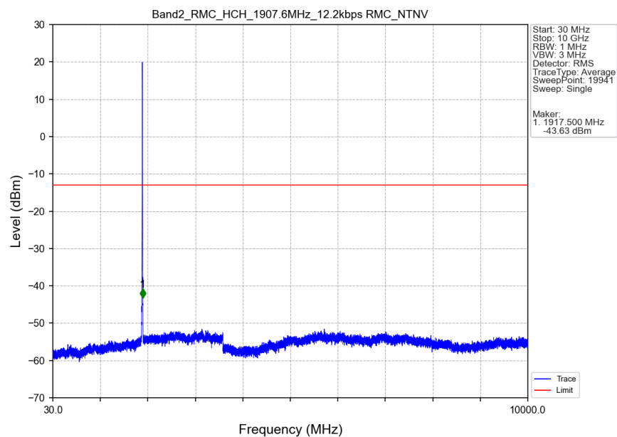
Band2_RMC_HCH_1907.6MHz_12.2kbps RMC_NTNV
