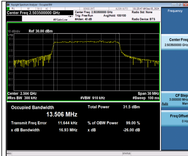
Band41-15MHz-QPSK-39725-75RB#0-PASS
