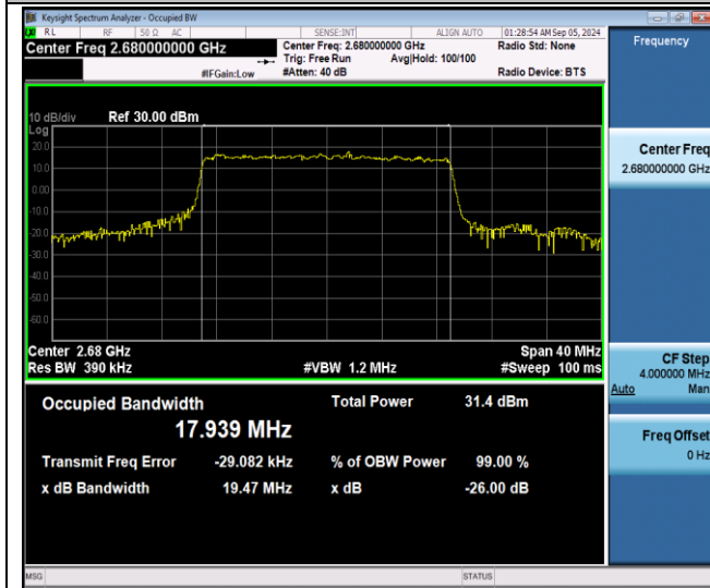
Band41-20MHz-QPSK-41490-100RB#0-PASS
