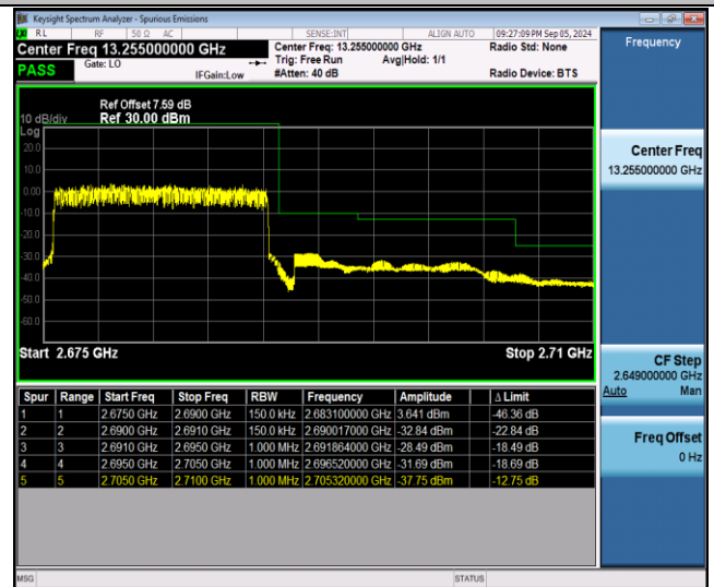
Band41-15MHz-QPSK-41515-75RB#0-PASS
