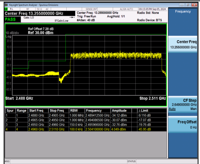
Band41-15MHz-QPSK-39725-75RB#0-PASS
