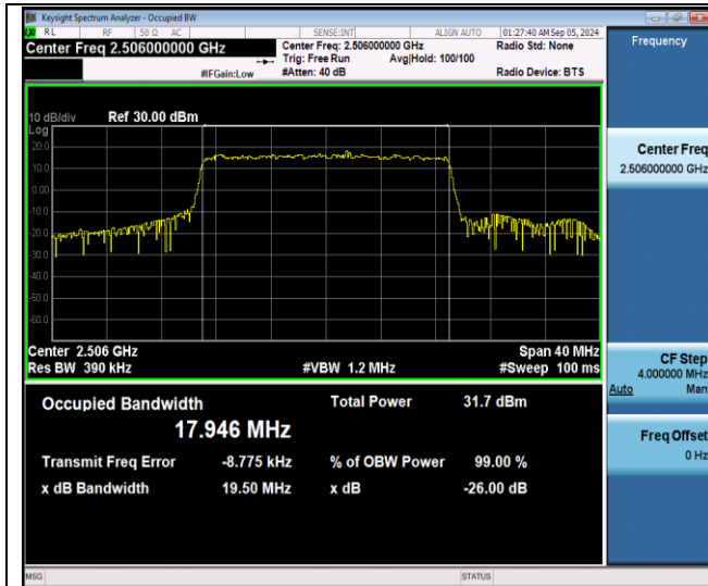
Band41-20MHz-QPSK-39750-100RB#0-PASS
