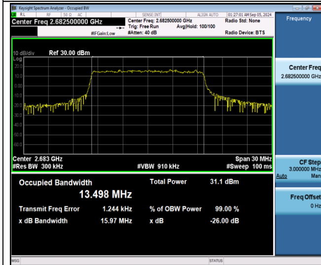
Band41-15MHz-QPSK-41515-75RB#0-PASS
