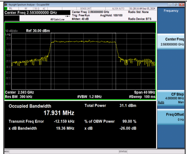
Band41-20MHz-QPSK-40620-100RB#0-PASS
