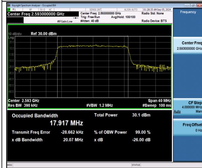
Band41-20MHz-16QAM-40620-100RB#0-PASS
