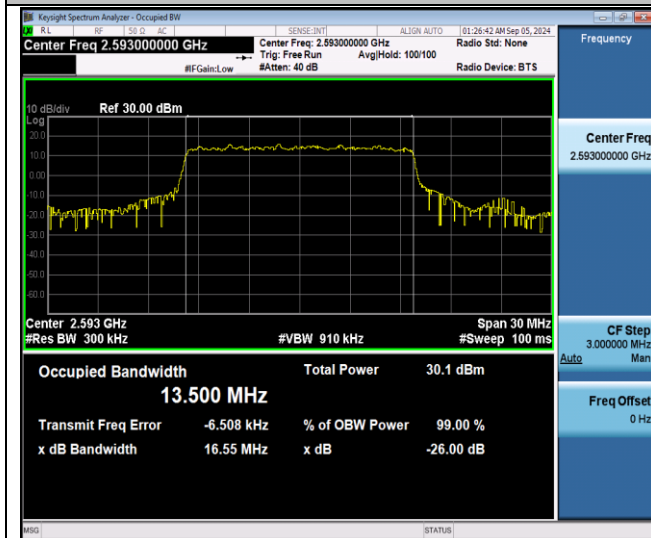
Band41-15MHz-16QAM-40620-75RB#0-PASS
