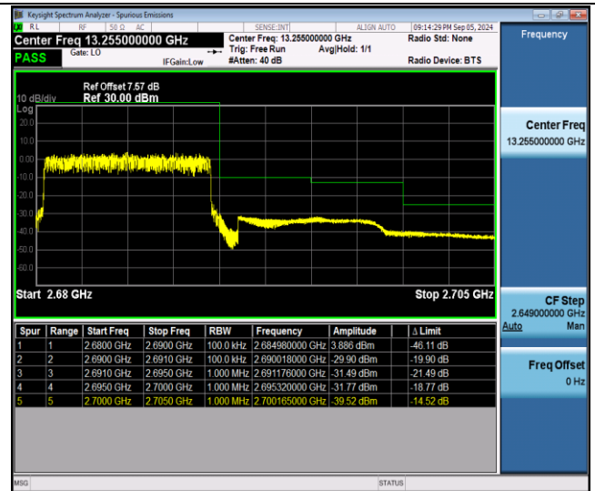
Band41-10MHz-QPSK-41540-50RB#0-PASS
