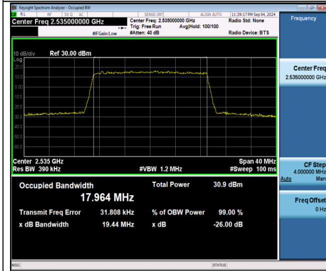
Band7-20MHz-16QAM-21100-100RB#0-PASS
