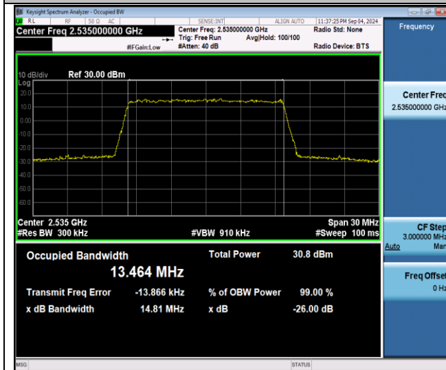
Band7-15MHz-16QAM-21100-75RB#0-PASS
