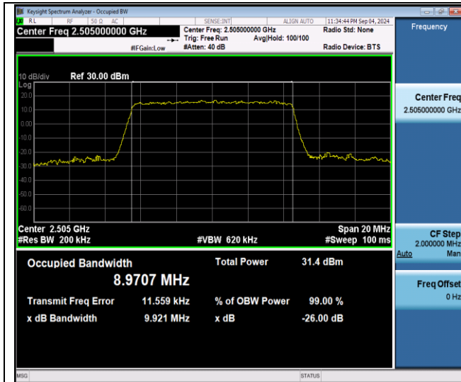
Band7-10MHz-QPSK-20800-50RB#0-PASS
