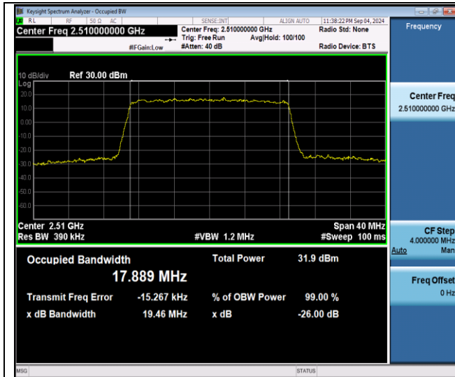
Band7-20MHz-QPSK-20850-100RB#0-PASS
