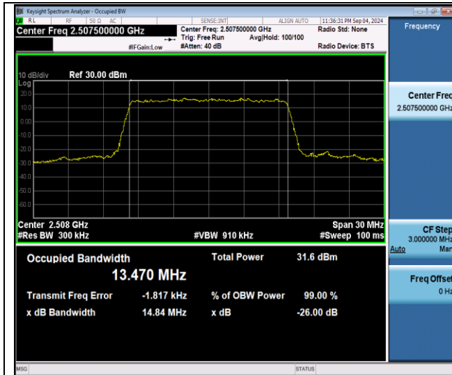
Band7-15MHz-QPSK-20825-75RB#0-PASS
