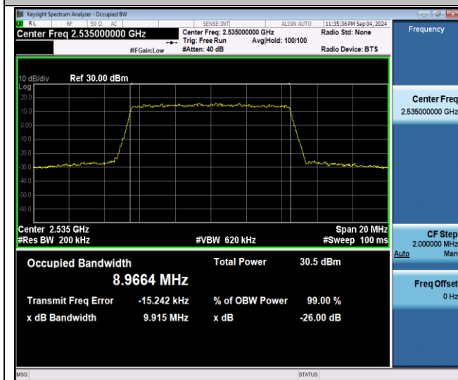
Band7-10MHz-16QAM-21100-50RB#0-PASS
