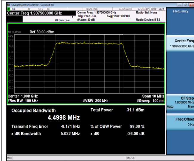
Band2-5MHz-QPSK-19175-25RB#0-PASS
