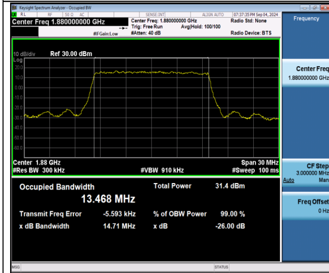
Band2-15MHz-16QAM-18900-75RB#0-PASS
