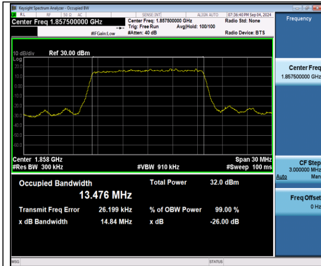
Band2-15MHz-QPSK-18675-75RB#0-PASS
