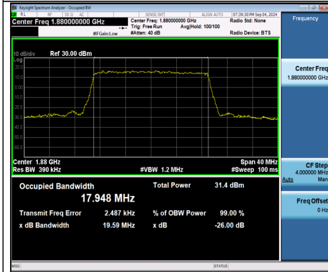
Band2-20MHz-16QAM-18900-100RB#0-PASS
