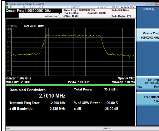
Band2-3MHz-QPSK-19085-15RB#0-PASS
