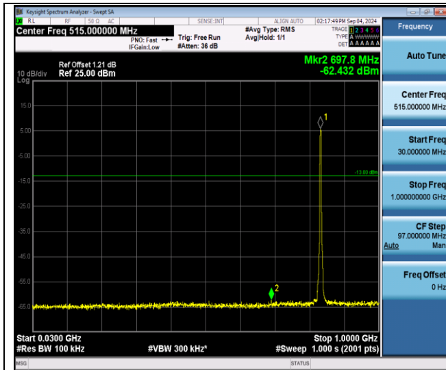
Band V-4182-30~1000MHz-PASS
