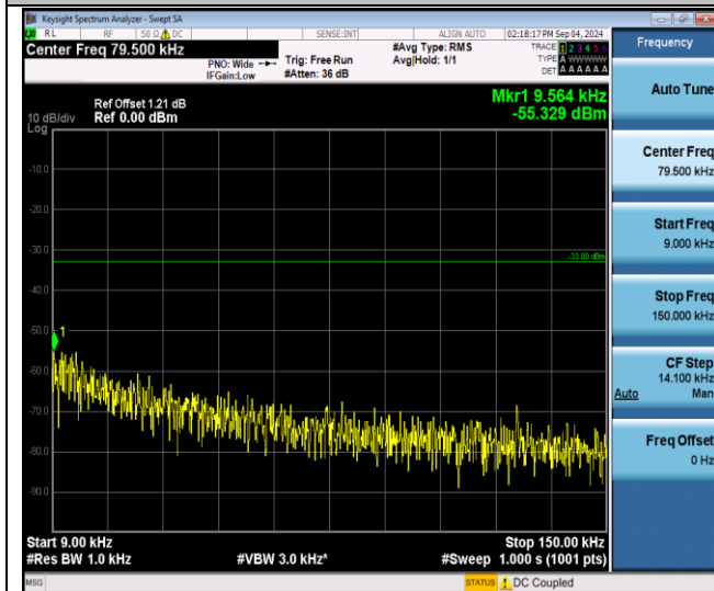
Band V-4233-0.009~0.15MHz-PASS
