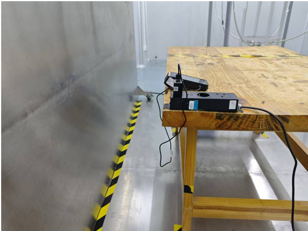
Conducted Emissions front View-M1-M5
