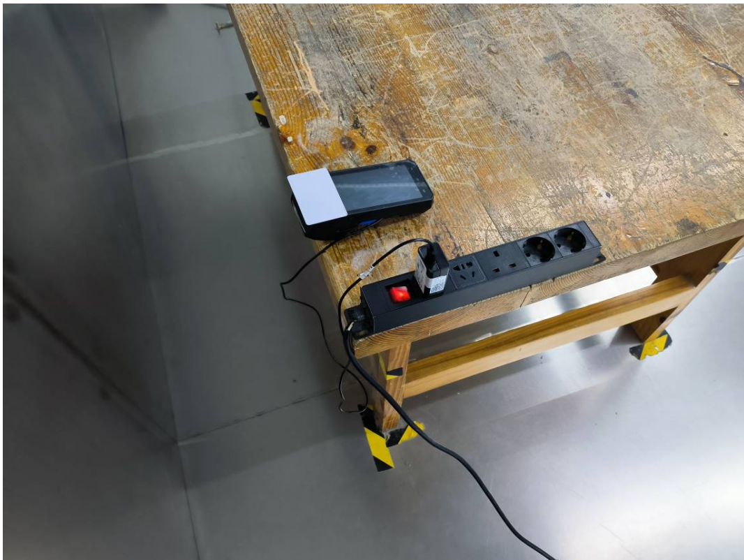
Conducted Emissions Side View Adapter 1# + IPS
