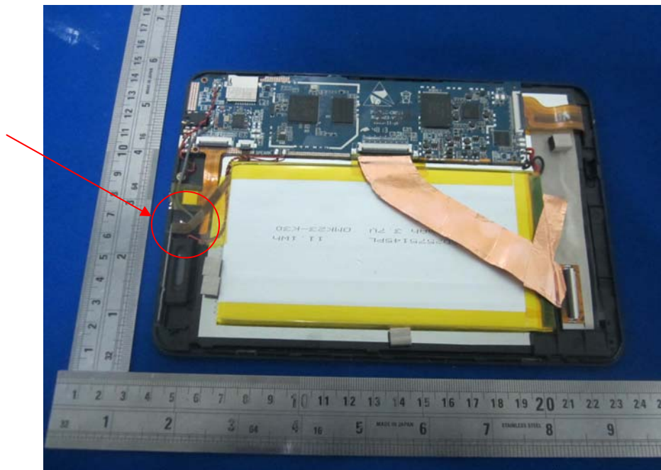
EUT- Back Cover Off and Shielding off View
