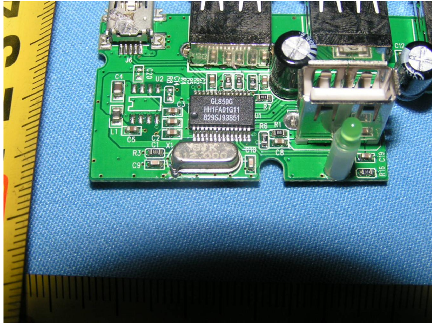
DX-B4PORT Main Board Chip View
