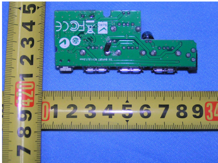
DX-B4PORT Main Board Soldered View
