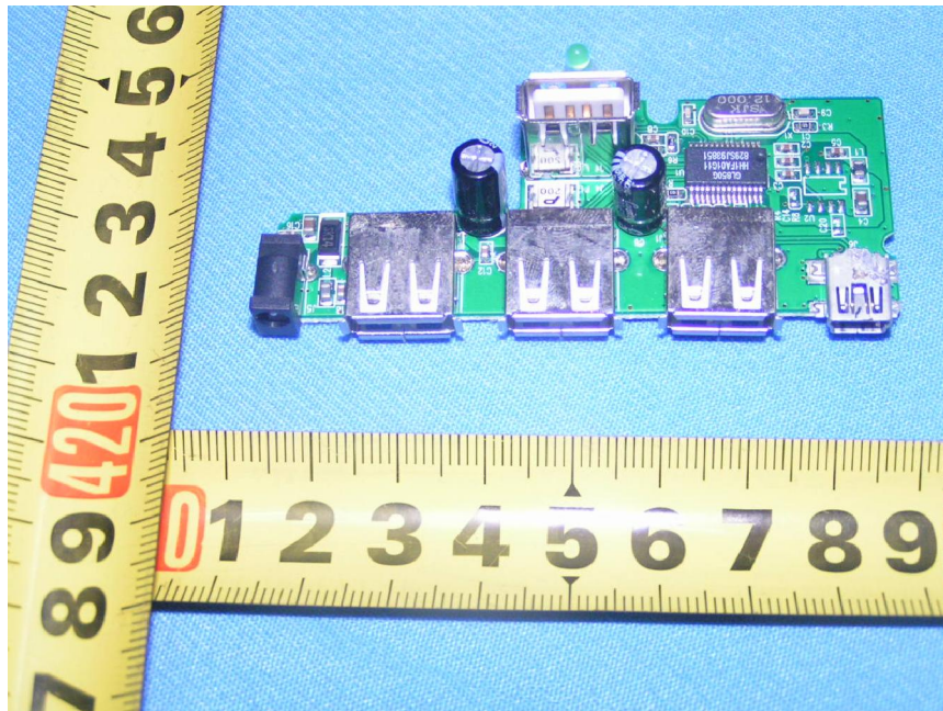
DX-B4PORT Main Board Component View
