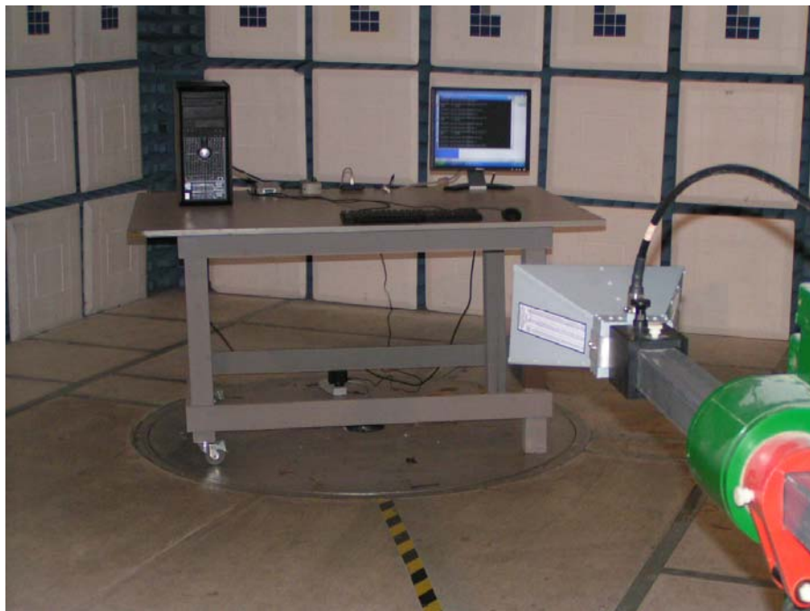
Radiated Emission High Frequency Test Set-Up View
