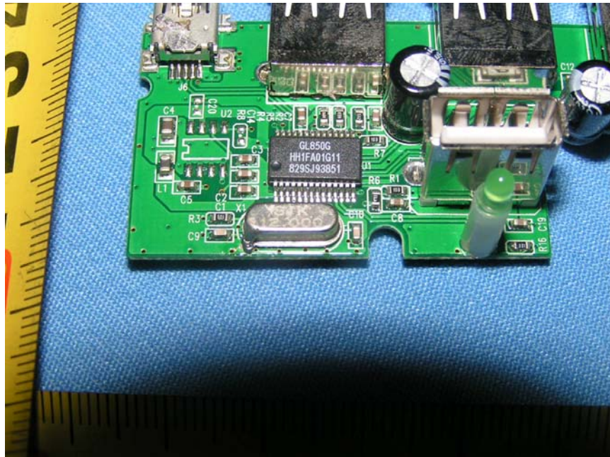
DX-B4PORT Main Board Chip View
