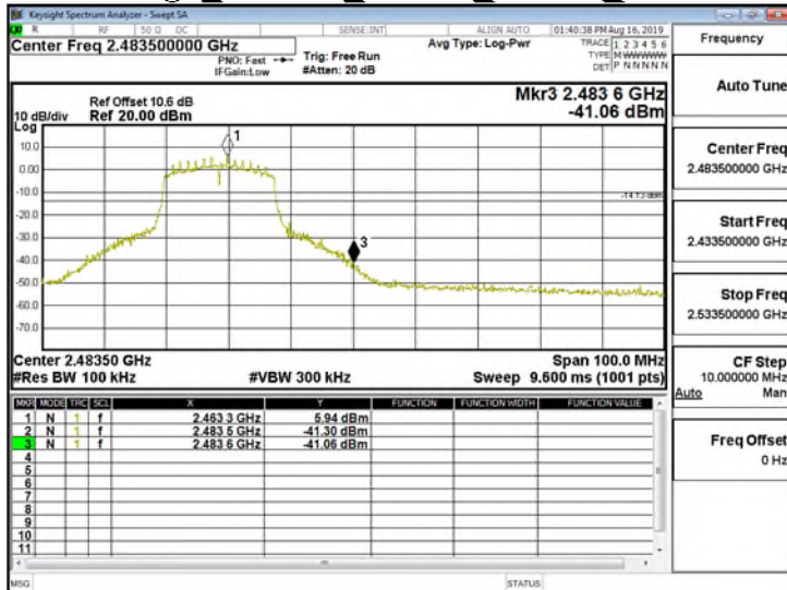
Band Edge_802.11n_20MHz_Chain0_2462MHz
