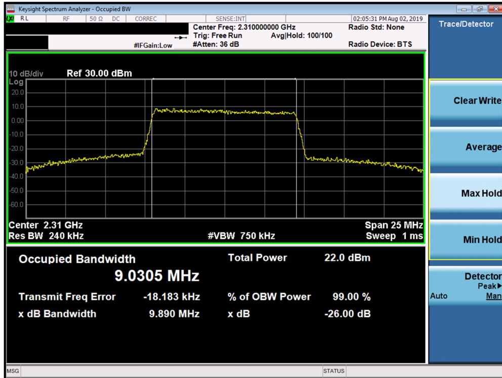
Plot 7-11. Occupied Bandwidth Plot (Band 30 - 10.0MHz 16-QAM - Full RB Configuration)
