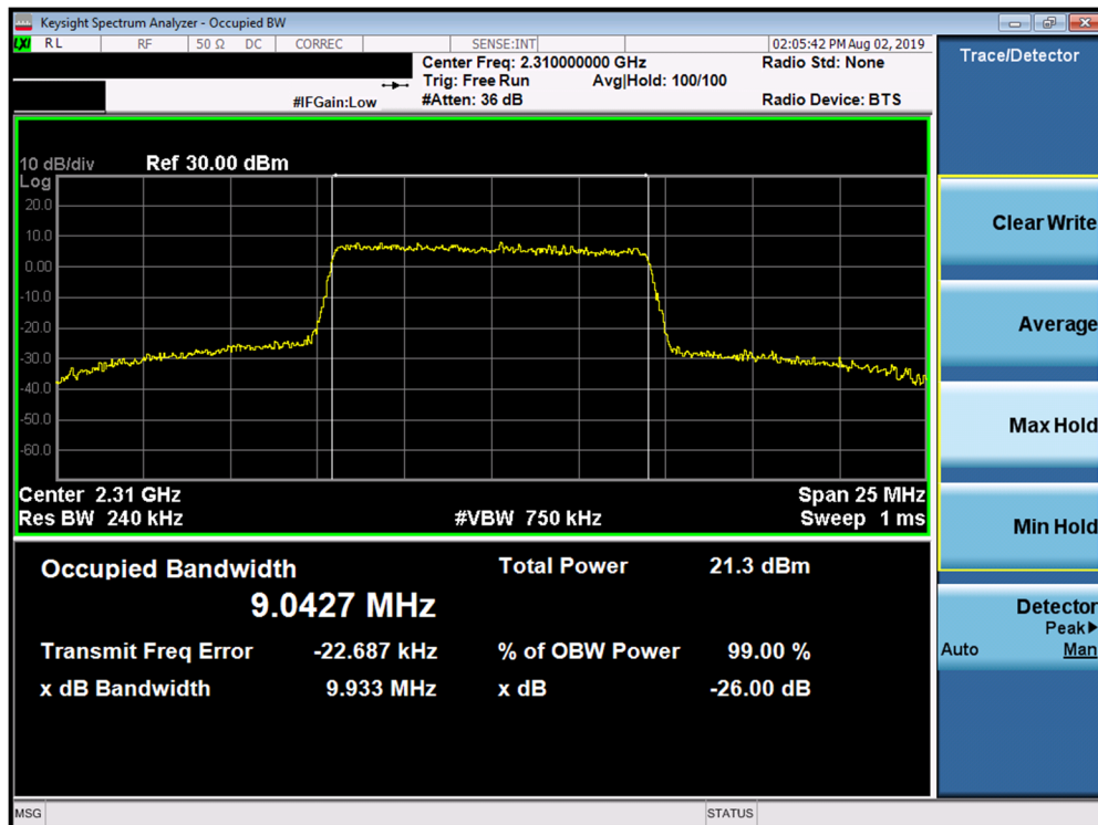
Plot 7-12. Occupied Bandwidth Plot (Band 30 - 10.0MHz 64-QAM - Full RB Configuration)
