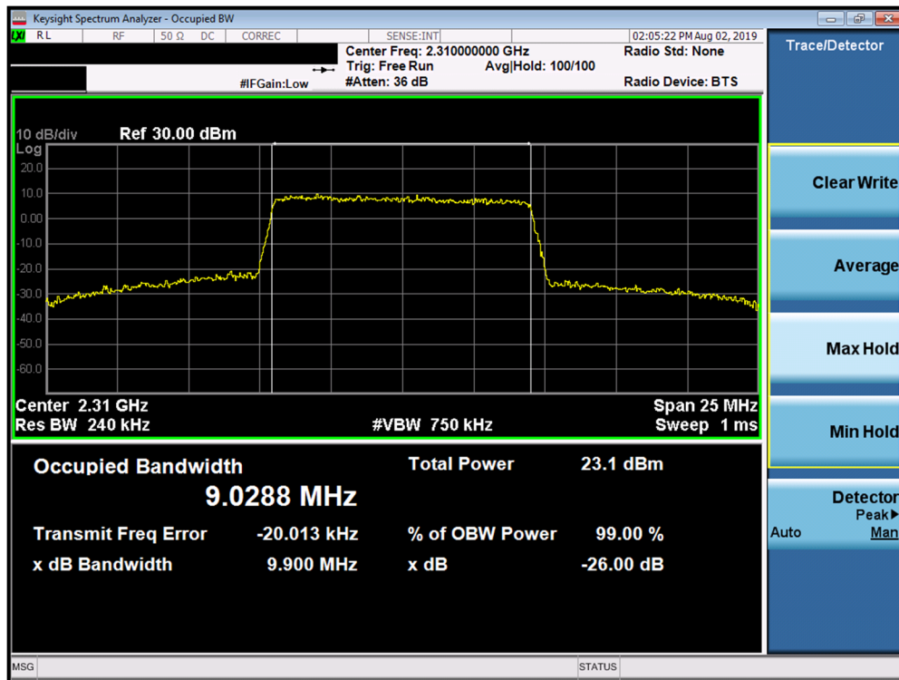
Plot 7-10. Occupied Bandwidth Plot (Band 30 - 10.0MHz QPSK - Full RB Configuration)
