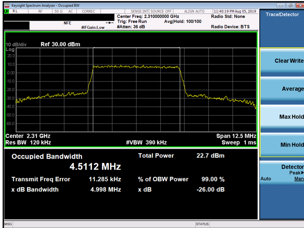
Plot 7-7. Occupied Bandwidth Plot (Band 30 - 5.0MHz QPSK - Full RB Configuration)
