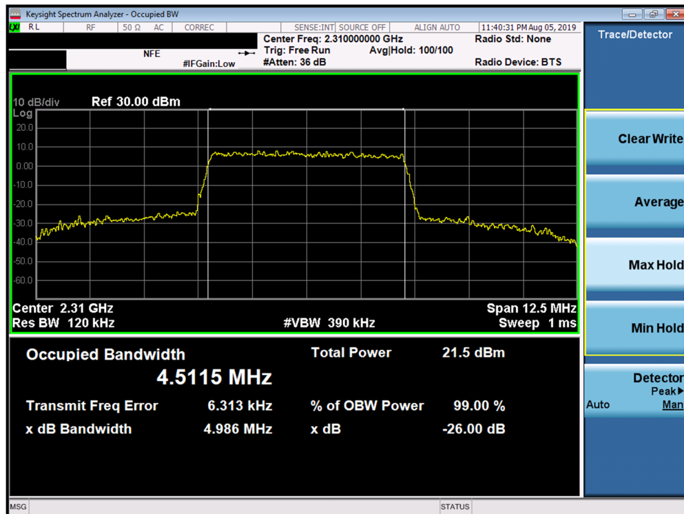
Plot 7-8. Occupied Bandwidth Plot (Band 30 - 5.0MHz 16-QAM - Full RB Configuration)
