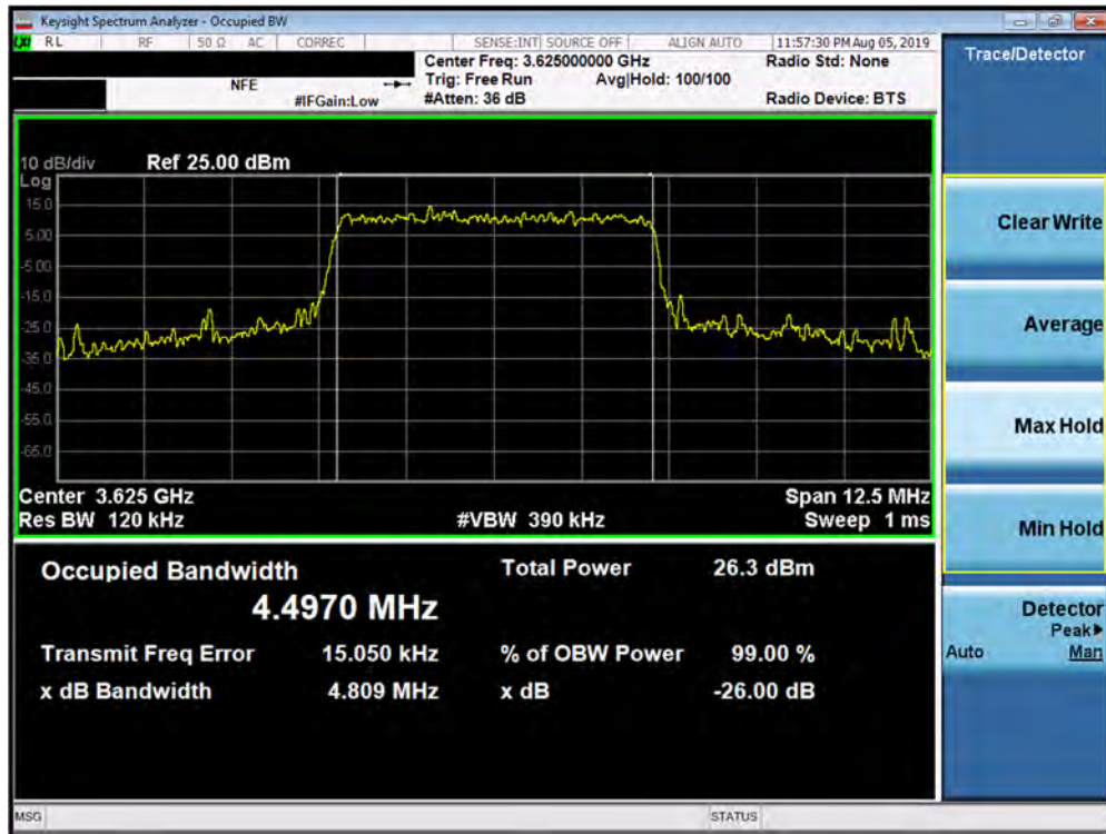
Plot 7-15. Occupied Bandwidth Plot (Band 48 - 5.0MHz 64-QAM - Full RB Configuration)
