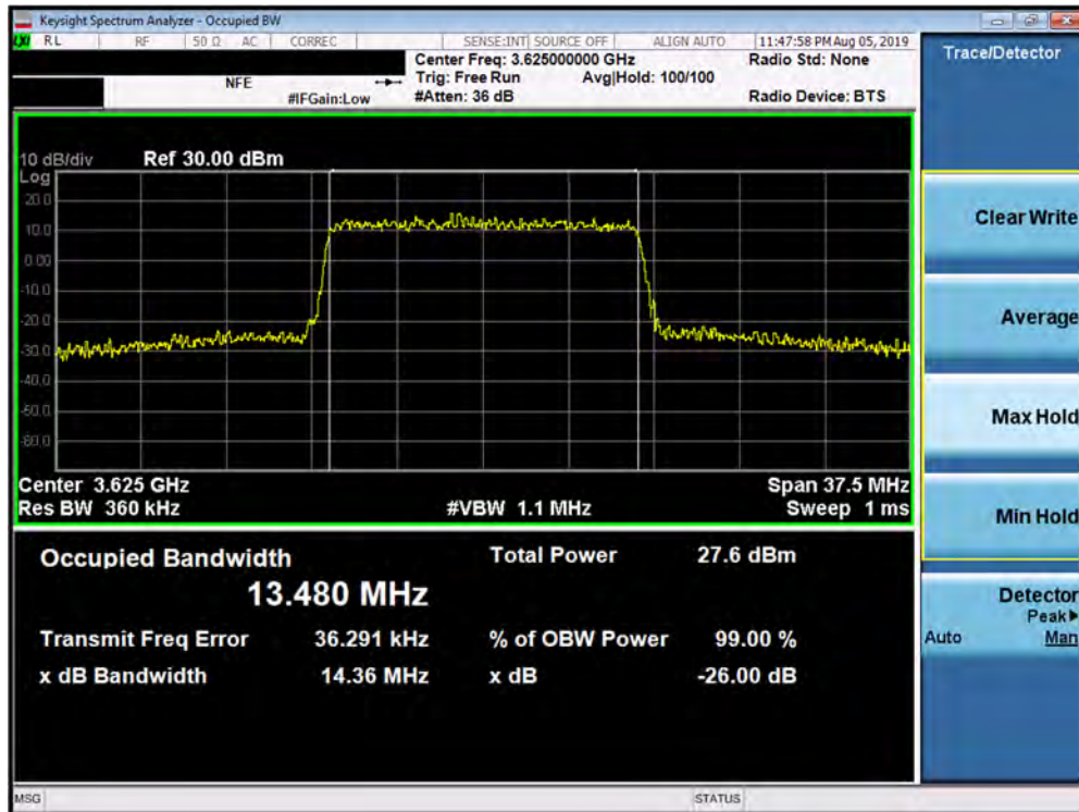
Plot 7-20. Occupied Bandwidth Plot (Band 48 - 15.0MHz 16-QAM - Full RB Configuration)
