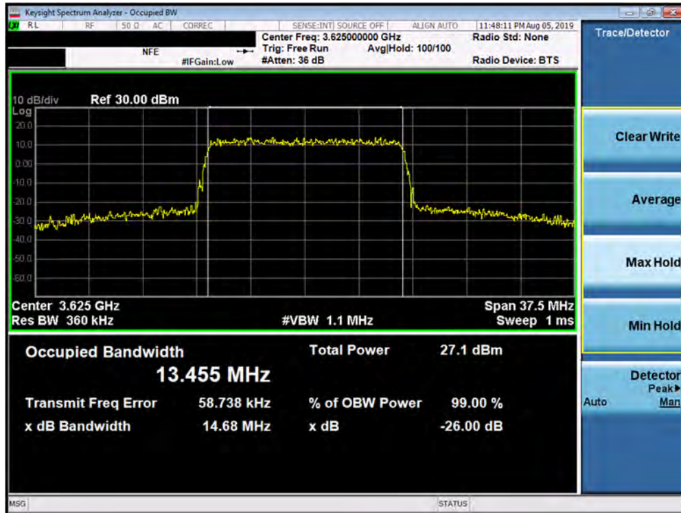
Plot 7-21. Occupied Bandwidth Plot (Band 48 - 15.0MHz 64-QAM - Full RB Configuration)
