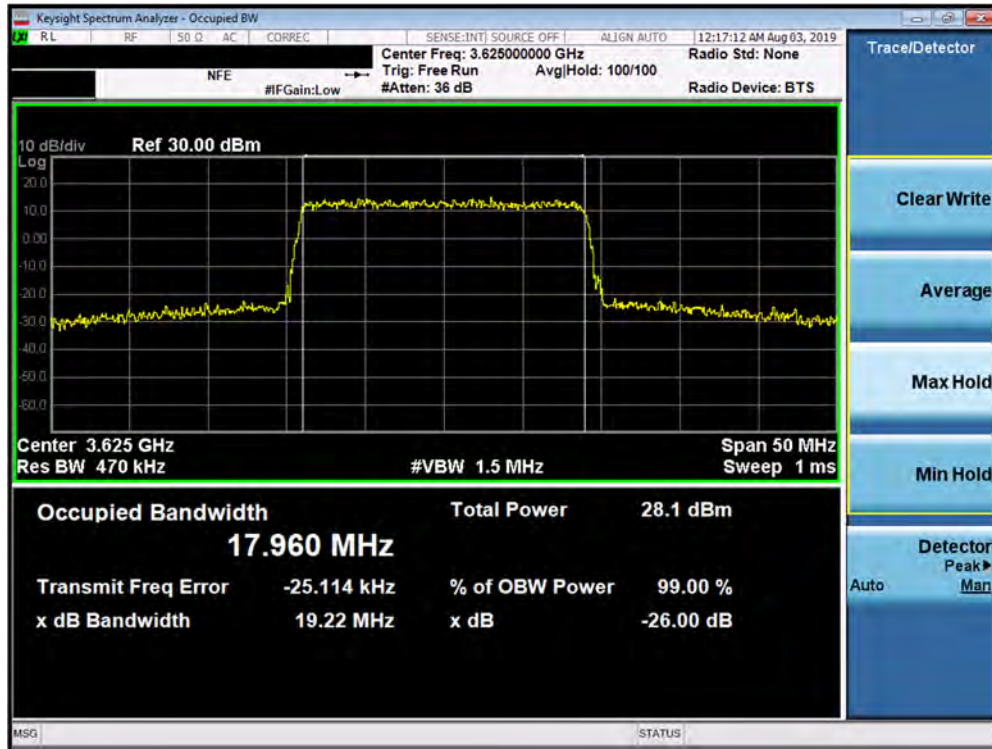
Plot 7-23. Occupied Bandwidth Plot (Band 48 - 20.0MHz 16-QAM - Full RB Configuration)
