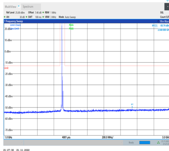
1-N70-PC3-15-15-H-1-DFT-PI2BPSK-Inner_1RB_Le ft-1@1-1000-3000-Ant1-2540.00--50.74--13-PASS
