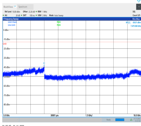
1-N70-PC3-15-15-H-1-DFT-PI2BPSK-Inner_1RB_Le ft-1@1-3000-18000-Ant1-7475.50--39.01--13-PASS
