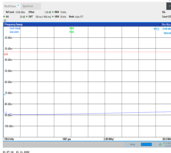
1-N70-PC3-15-15-H-1-DFT-PI2BPSK-Inner_1RB_Le ft-1@1-0.15-30-Ant1-0.15--74.99--33-PASS
