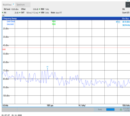
1-N70-PC3-15-15-H-1-DFT-PI2BPSK-Inner_1RB_Le ft-1@1-0.009-0.15-Ant1-0.06--69.18--43-PASS
