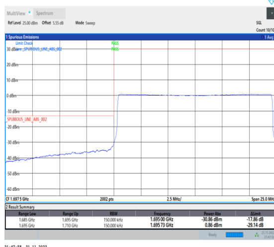
1-N70-PC3-15-15-L-6-CP-QPSK-Outer_Full-79@0-Ant1-1-seegraph-PASS-see graph
