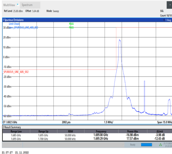
1-N70-PC3-15-5-L-1-DFT-PI2BPSK-Edge_1RB_Left-1 @0-Ant1-1-seegraph-PASS-see graph
