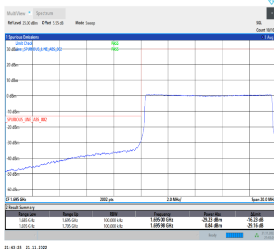
1-N70-PC3-15-10-L-6-CP-QPSK-Outer_Full-52@0-Ant1-1-seegraph-PASS-see graph
