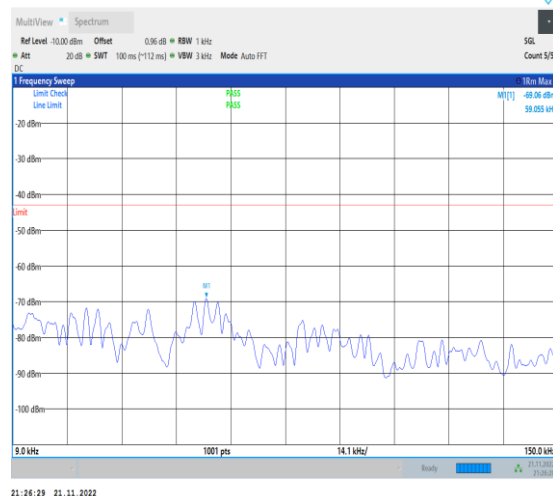
1-N70-PC3-15-15-M-1-DFT-PI2BPSK-Inner_1RB_Le ft-1@1-0.009-0.15-Ant1-0.06--69.06--43-PASS
