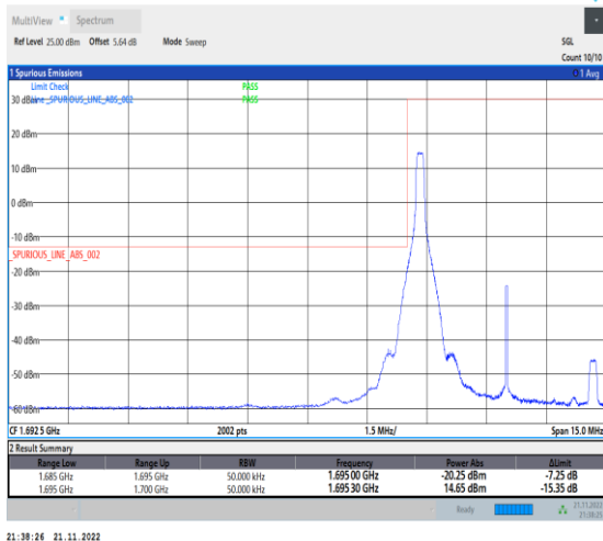
1-N70-PC3-15-5-L-4-CP-QPSK-Edge_1RB_Left-1@0-Ant1-1-seegraph-PASS-see graph
