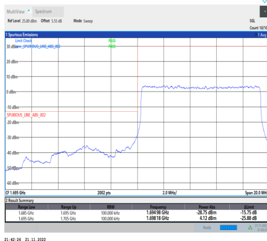
1-N70-PC3-15-10-L-3-DFT-PI2BPSK-Outer_Full-50@0-Ant1-1-seegraph-PASS-see graph
