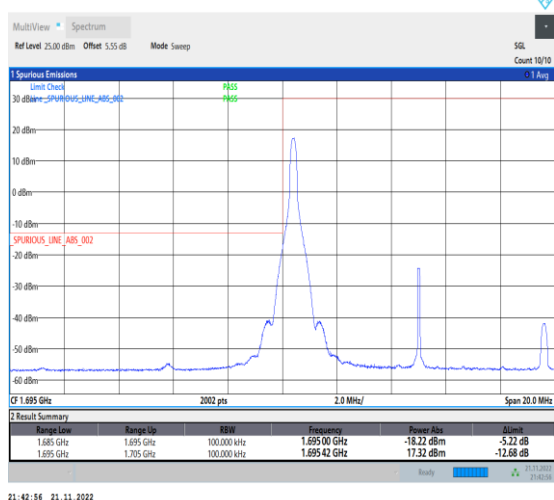
1-N70-PC3-15-10-L-4-CP-QPSK-Edge_1RB_Left-1@0-Ant1-1-seegraph-PASS-see graph
