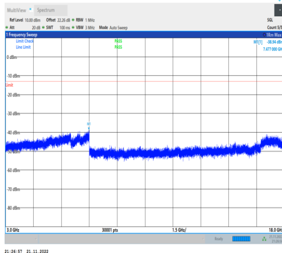
1-N70-PC3-15-15-M-1-DFT-PI2BPSK-Inner_1RB_Le ft-1@1-3000-18000-Ant1-7477.00--38.94--13-PASS
