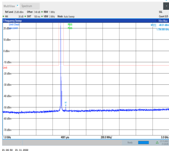
1-N70-PC3-15-15-M-1-DFT-PI2BPSK-Inner_1RB_Le ft-1@1-1000-3000-Ant1-1756.50--49.31--13-PASS
