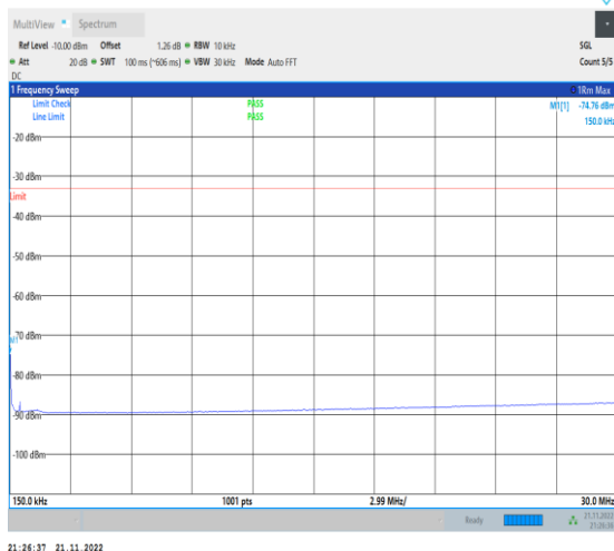
1-N70-PC3-15-15-M-1-DFT-PI2BPSK-Inner_1RB_Le ft-1@1-0.15-30-Ant1-0.15--74.76--33-PASS
