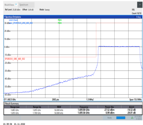
1-N70-PC3-15-5-L-6-CP-QPSK-Outer_Full-25@0-Ant1-1-seegraph-PASS-see graph
