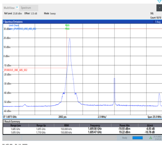
1-N70-PC3-15-15-L-4-CP-QPSK-Edge_1RB_Left-1@0-Ant1-1-seegraph-PASS-see graph
