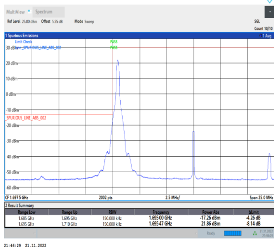
1-N70-PC3-15-15-L-1-DFT-PI2BPSK-Edge_1RB_Left-1@0-Ant1-1-seegraph-PASS-see graph
