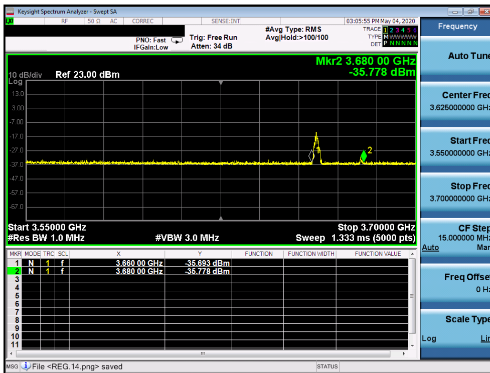
Plot 7. Conducted Measurement – UUT RF transmission range and bandwidths are less or equal to frequency range and bandwidth of compatible BTS-CBSD(WINNF.FT.C.REG.16)
