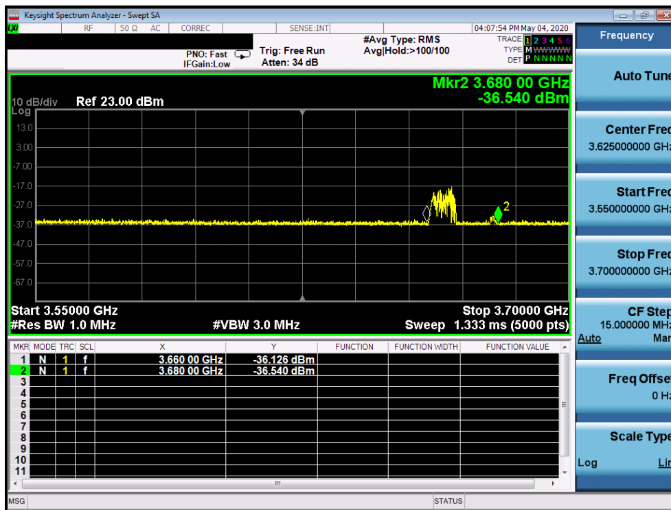
Plot 17. Conducted Measurement – UUT RF transmission range and bandwidths are less or equal to frequency range and bandwidth of compatible BTS-CBSD (WINNF.TT.C.HBT.9)
