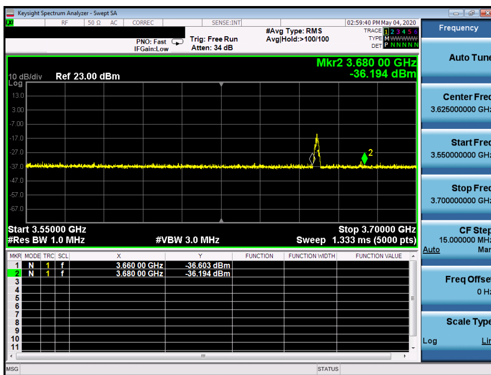
Plot 4. Conducted Measurement – UUT RF transmission range and bandwidths are less or equal to frequency range and bandwidth of compatible BTS-CBSD(WINNF.FT.C.REG.10)
