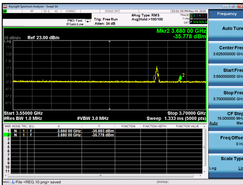
Plot 5. Conducted Measurement – UUT RF transmission range and bandwidths are less or equal to frequency range and bandwidth of compatible BTS-CBSD(WINNF.FT.C.REG.12)
