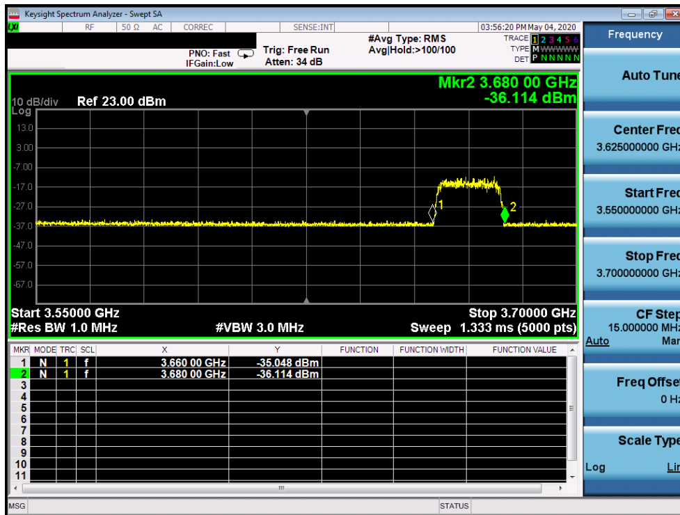
Plot 15. Conducted Measurement – UUT RF transmission range and bandwidths are less or equal to frequency range and bandwidth of compatible BTS-CBSD (WINNF.TT.C.HBT.6)
