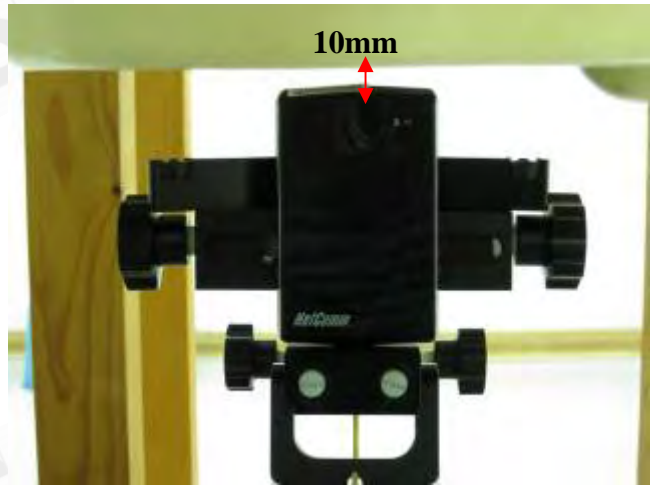
Fig.5 Top side of EUT is paralleled with flat phantom and spacing between EUT and Phantom is 10mm.
