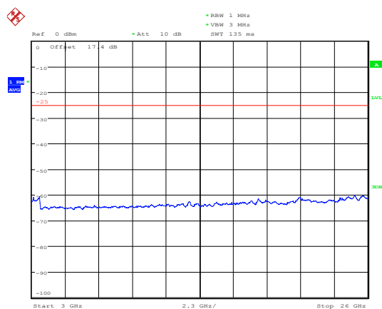
LTE Band 7 5MHz CH-Low 3GHz~26GHz
