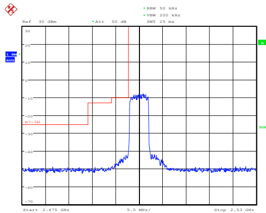
LTE Band 7 16QAM 5MHz CH-Low, 100%RB
