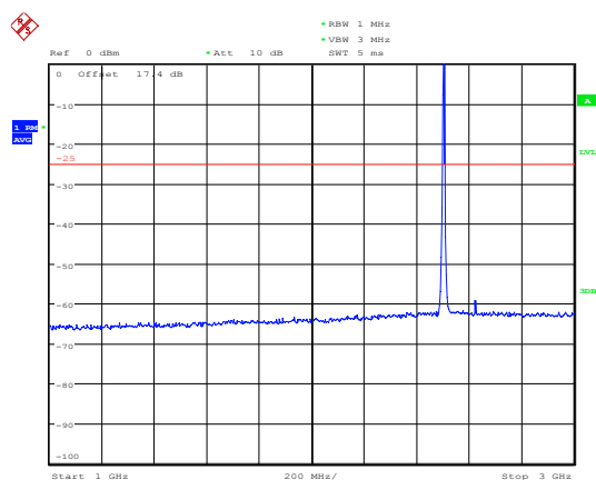
LTE Band 7 5MHz CH-Low 1GHz~3GHz
