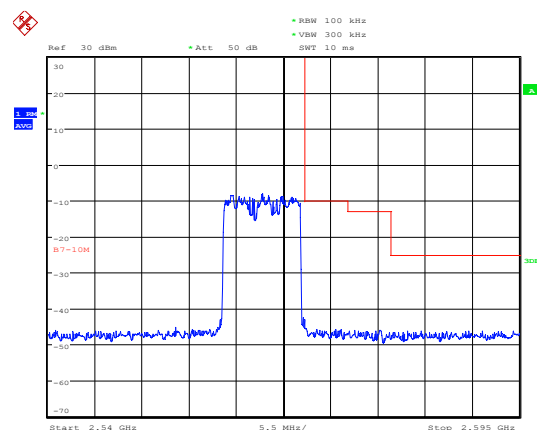
LTE Band 7 16QAM 10MHz CH-High, 100%RB
