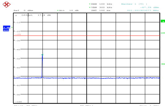
LTE Band 7 5MHz CH-Middle 30MHz~1GHz
