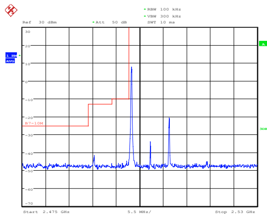
LTE Band 7 16QAM 10MHz CH-Low, 1 RB
