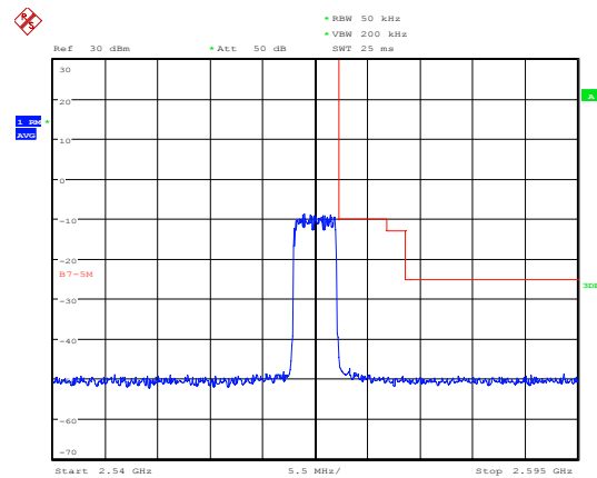
LTE Band 7 16QAM 5MHz CH-High, 100%RB
