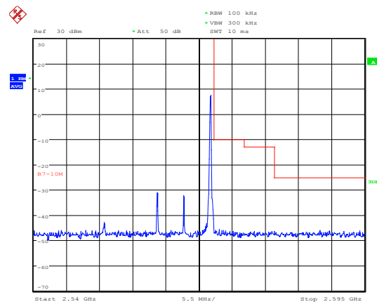
LTE Band 7 16QAM 10MHz CH-High, 1 RB
