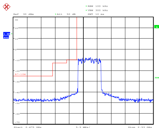
LTE Band 7 16QAM 10MHz CH-Low, 100%RB
