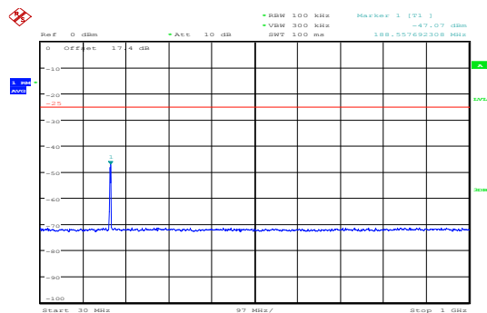
LTE Band 7 5MHz CH-Low 30MHz~1GHz
