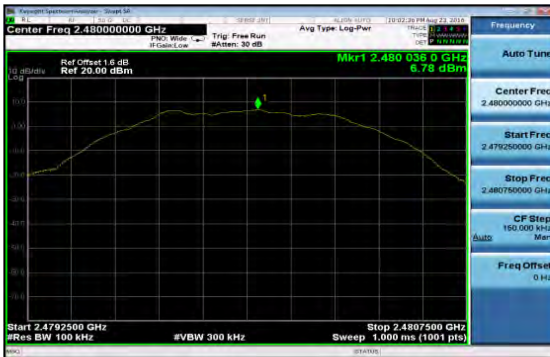
Power Spectral Density for Bandedge Limit (CH-High)
