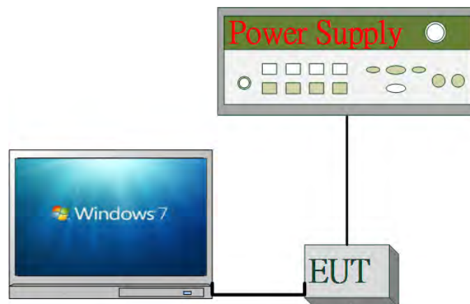
Fig. 2-1 Conducted Emission
