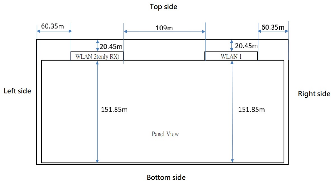
Fig.8 Antenna location of EUT
