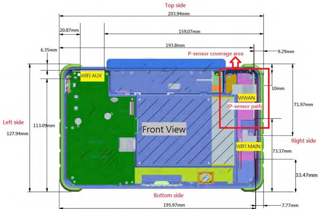
Fig.14 Antenna position of EUT (Front view)
