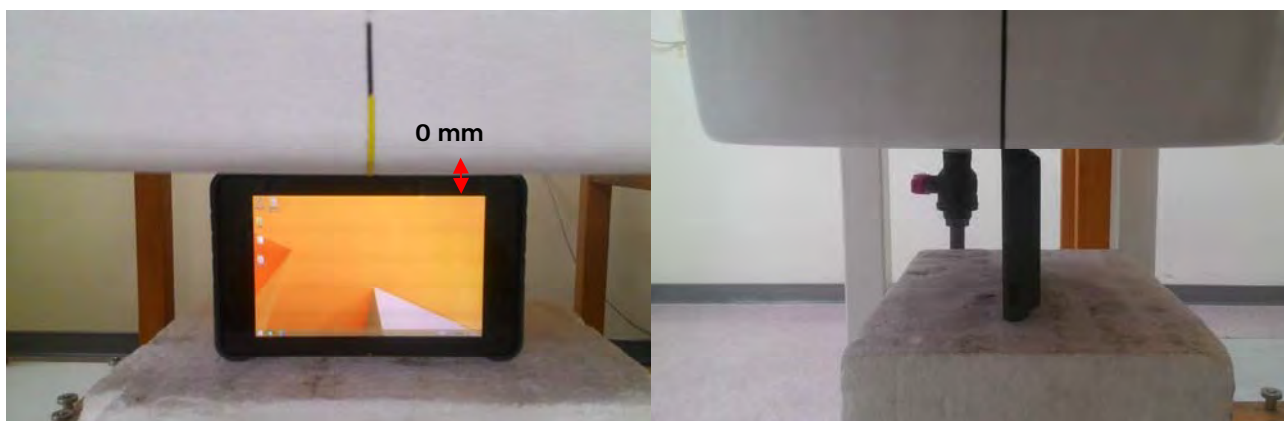
Fig.4 EUT Bottom side to flat phantom
