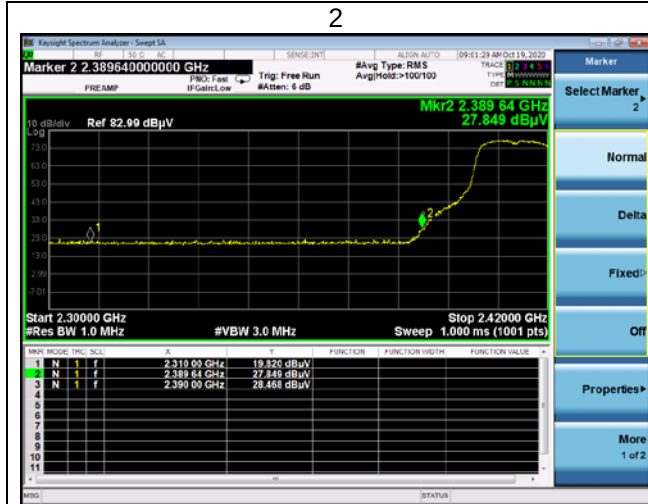
Low channel (Peak)
