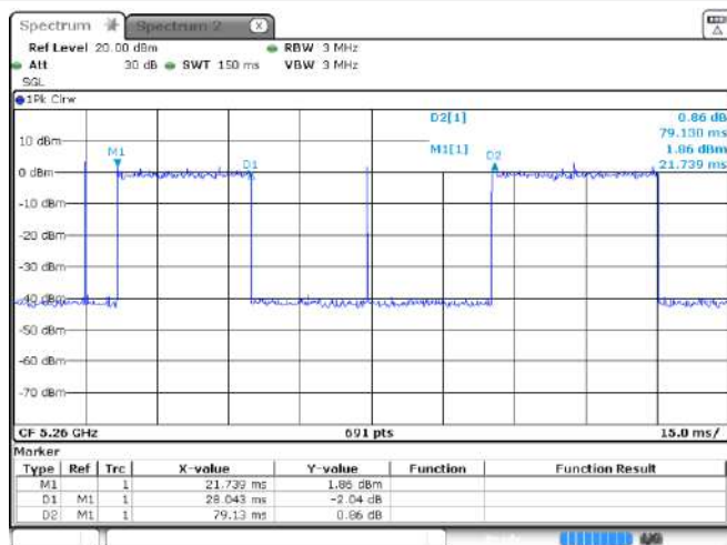
11a 5260 MHz
