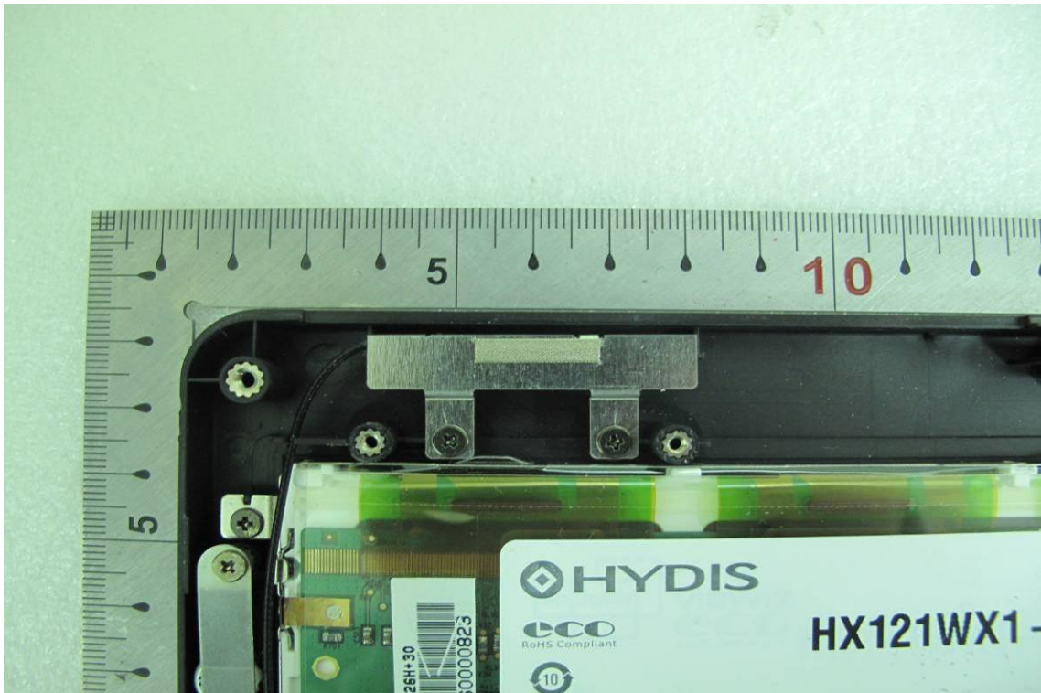
Internal View of EUT -10 (WLAN Antenna Main)
