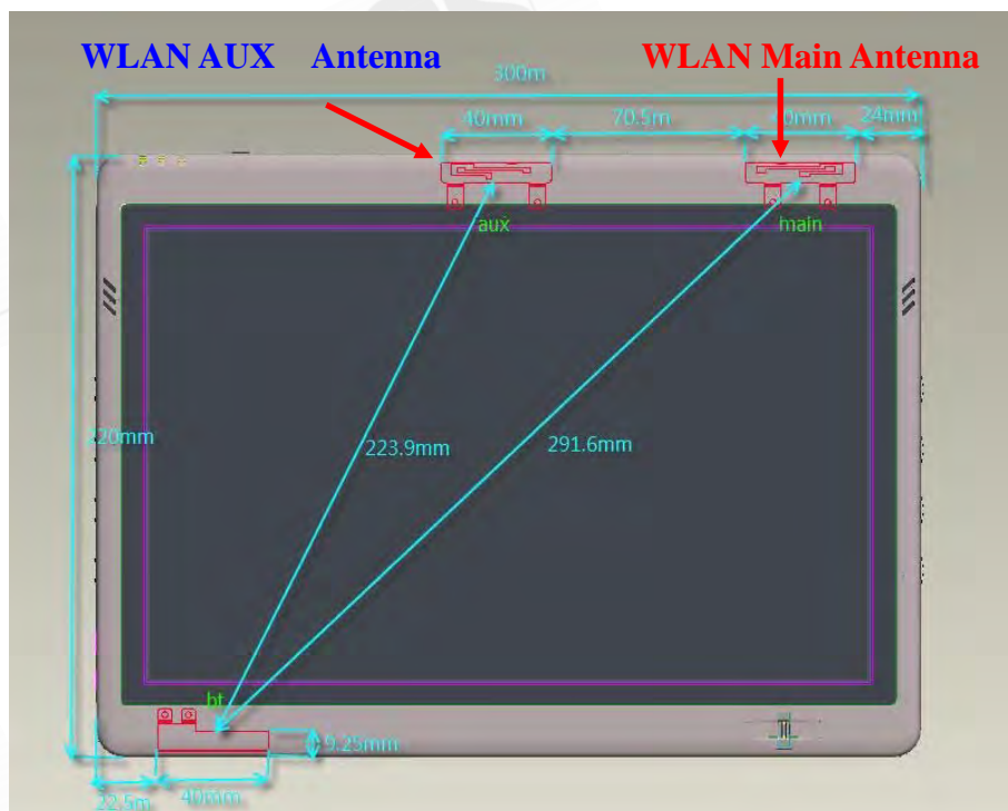
Fig.3 Antenna position of EUT
