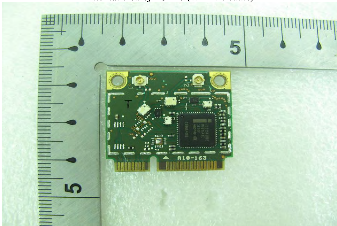
Internal View of EUT – 5 (WLAN Module)
