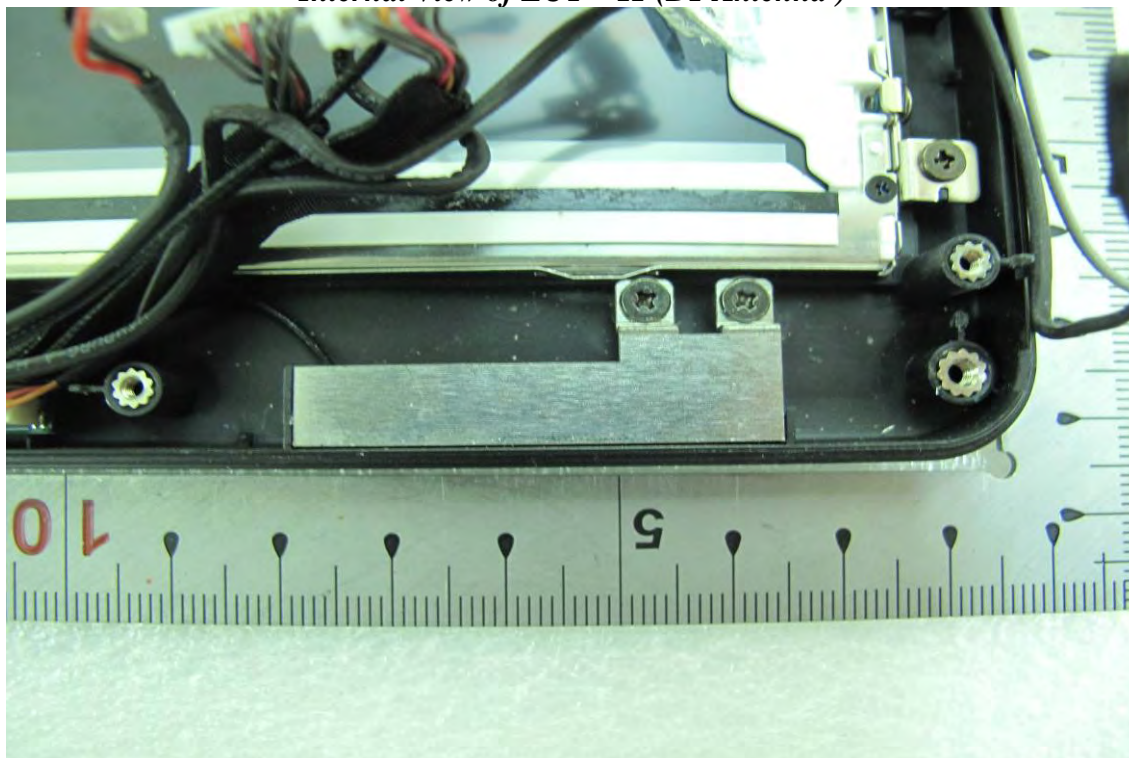
Internal View of EUT - 11 (BT Antenna )
