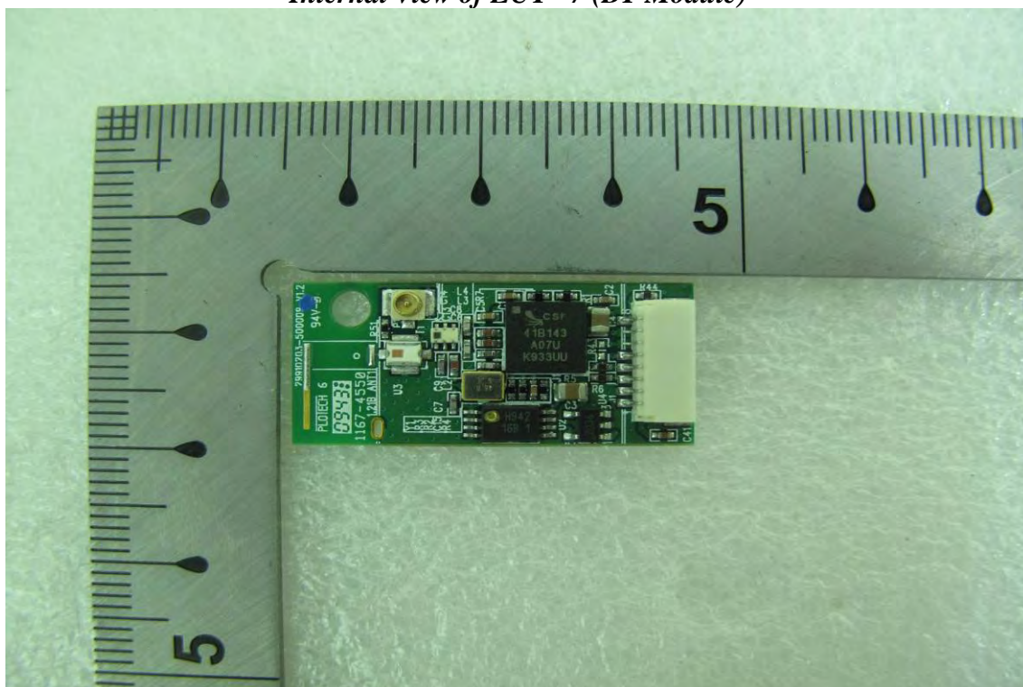
Internal View of EUT – 7 (BT Module)
