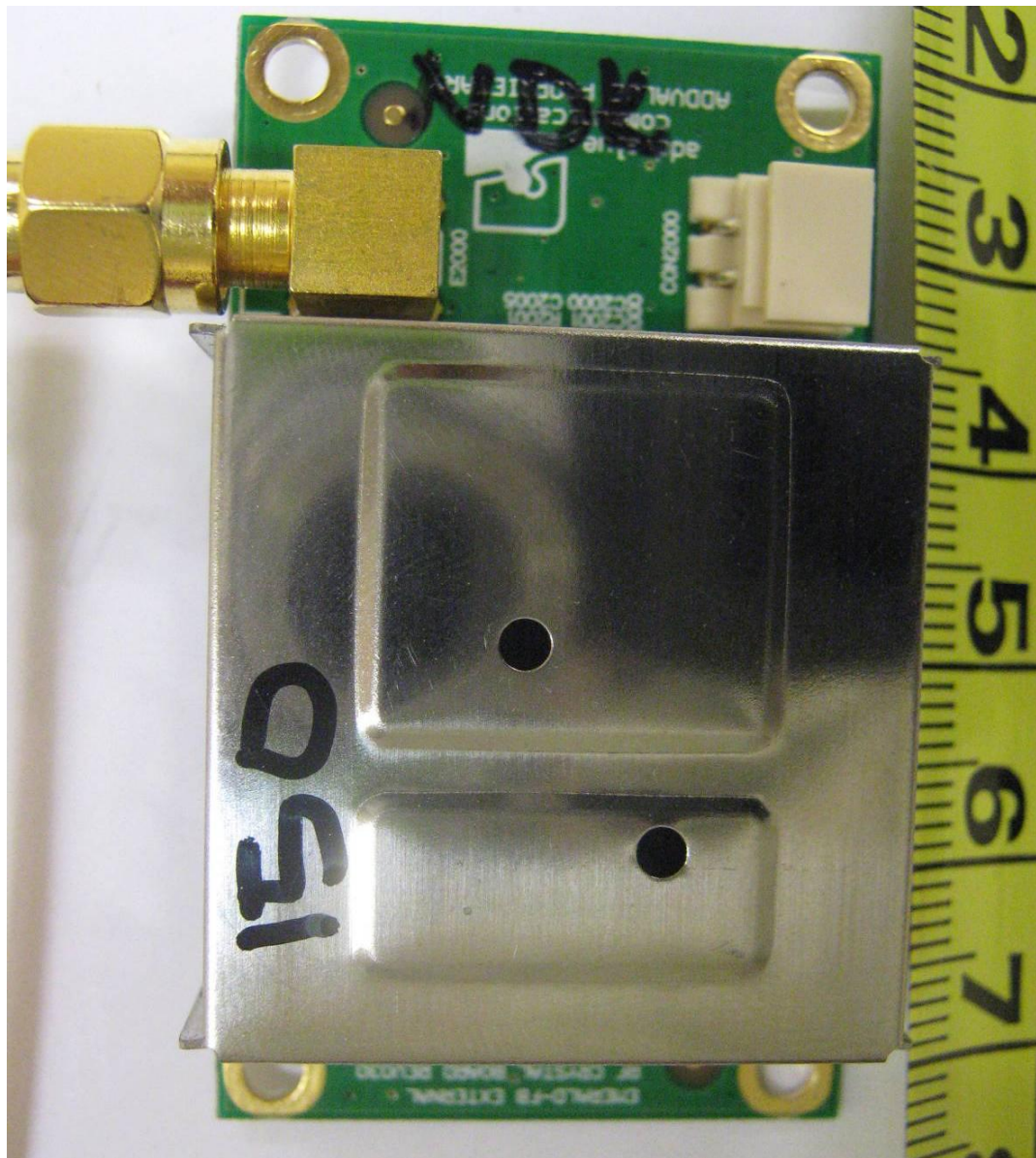
Crystal Board Component Side
