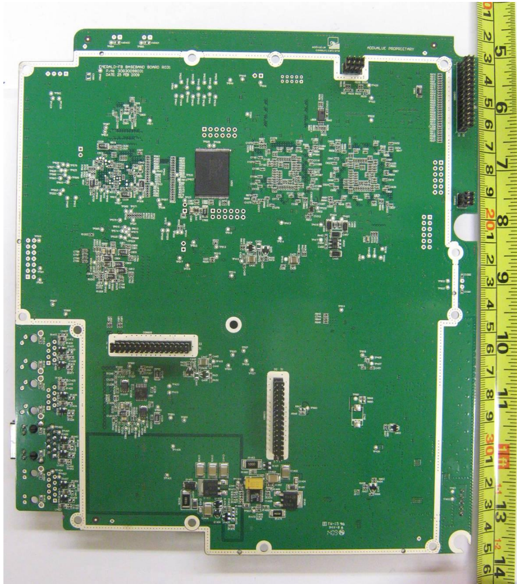
Base-Band Board PCB Trace Side
