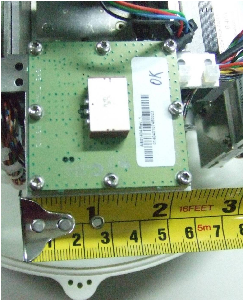
PCB View 2
