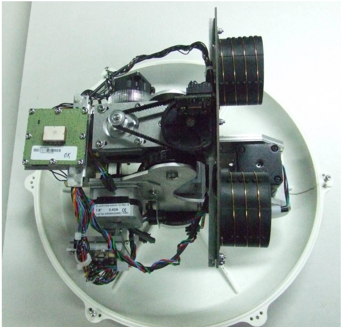
Internal View 2
