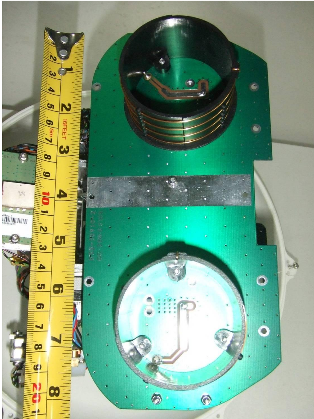
PCB View 1
