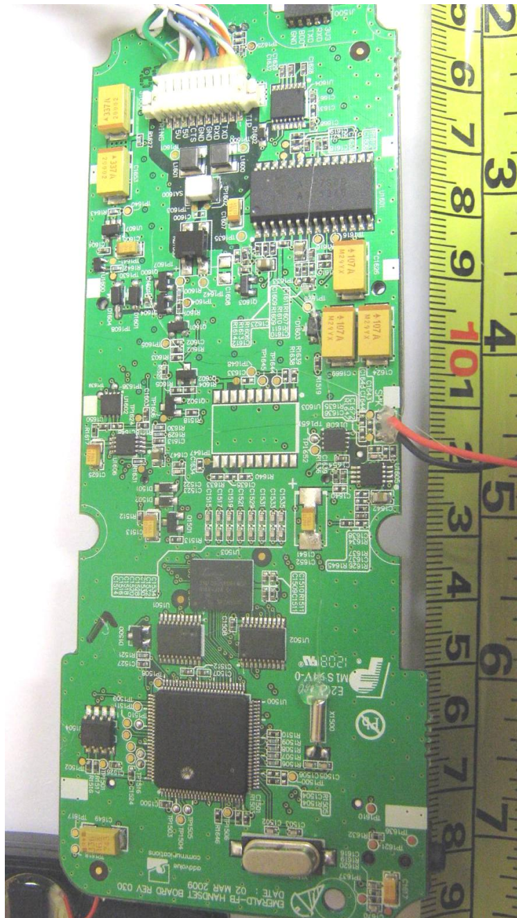
Main-Board Component Side
