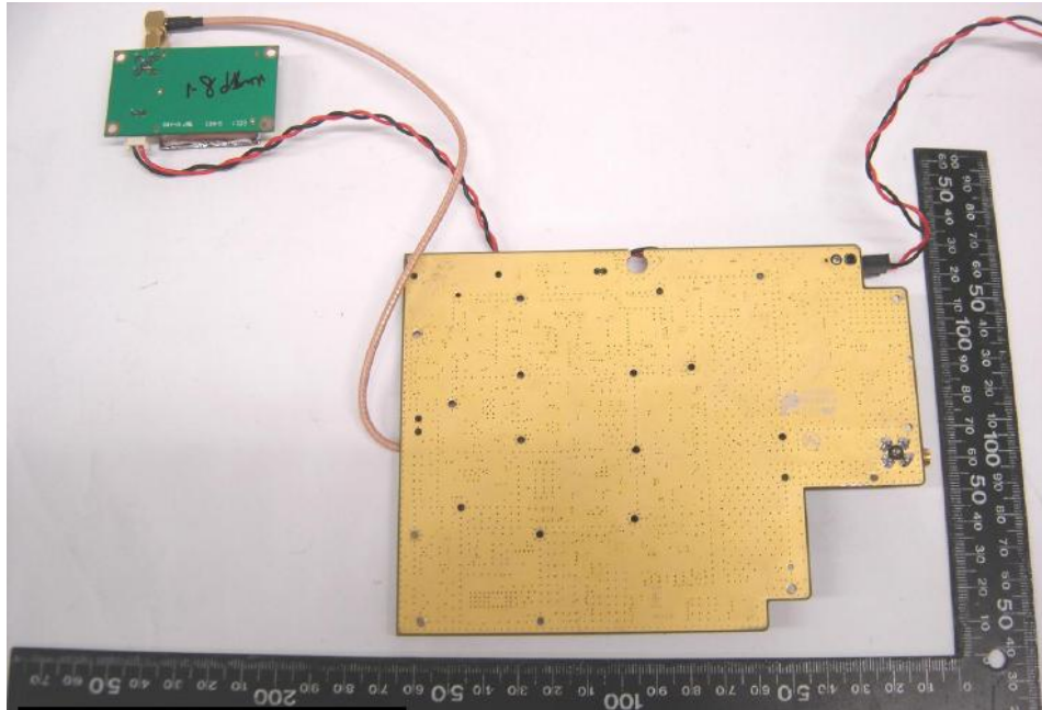
PCB views "RF Board" of Fleet Broadband Satellite Communication System
