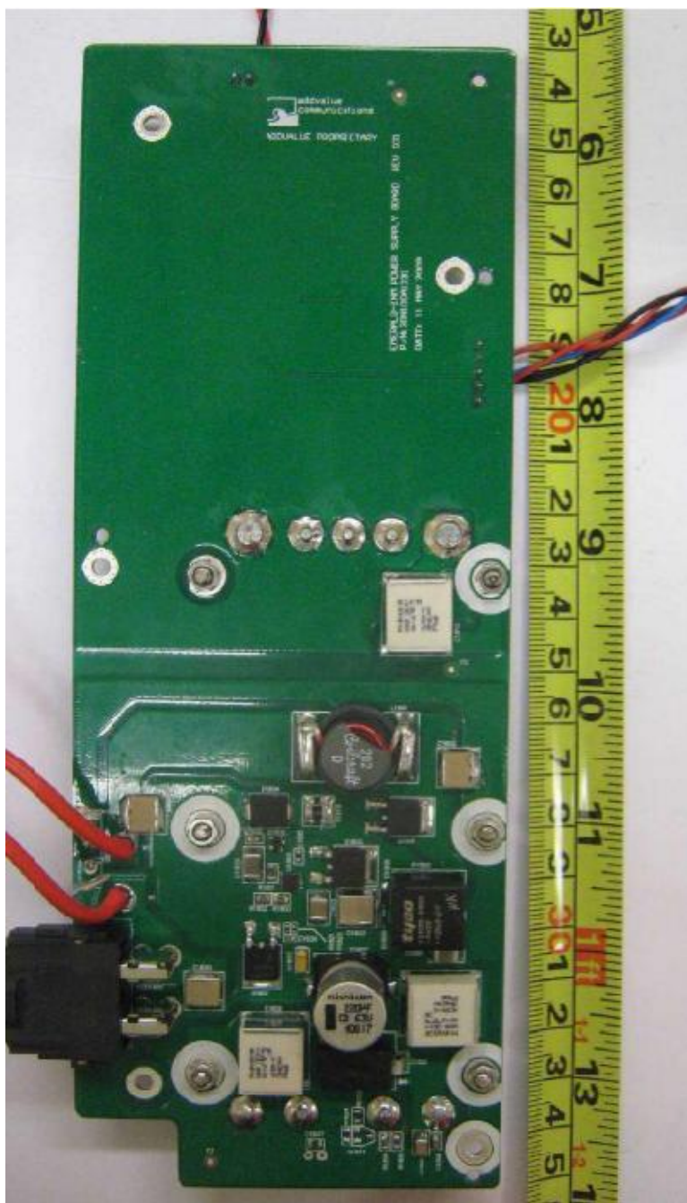
Power Supply Board PCB Trace Side
