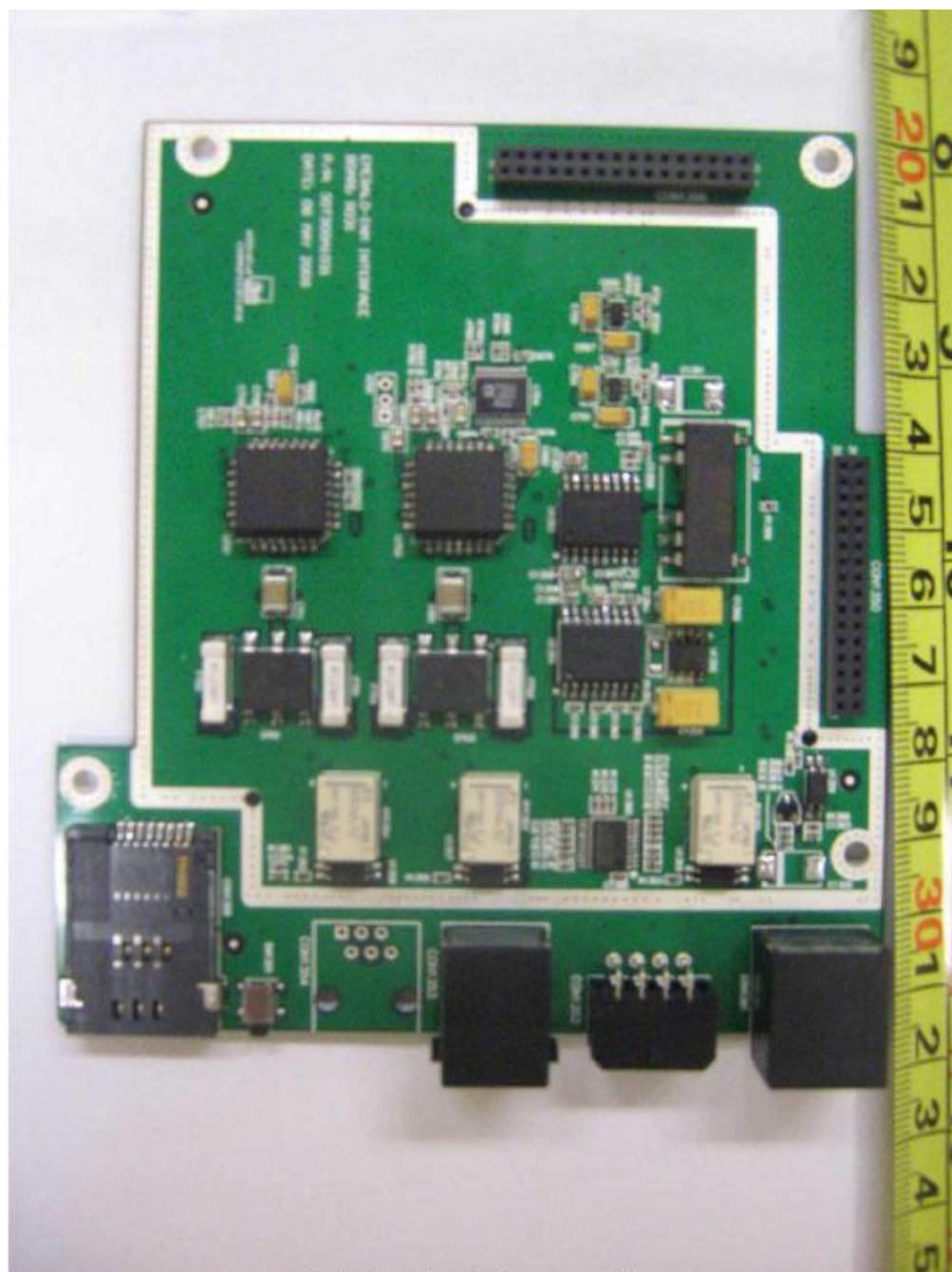
Interface Board Component Side
