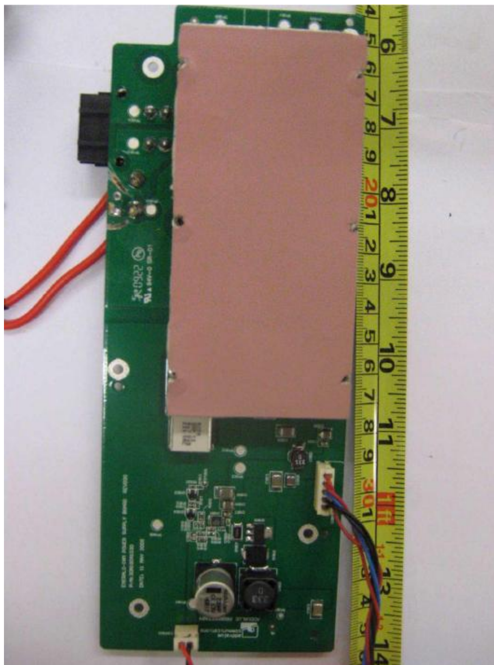
Power Supply Board Component Side
