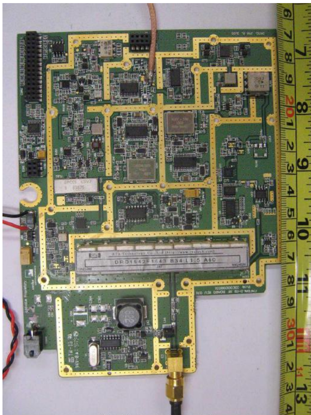
RF Module Board Component Side
