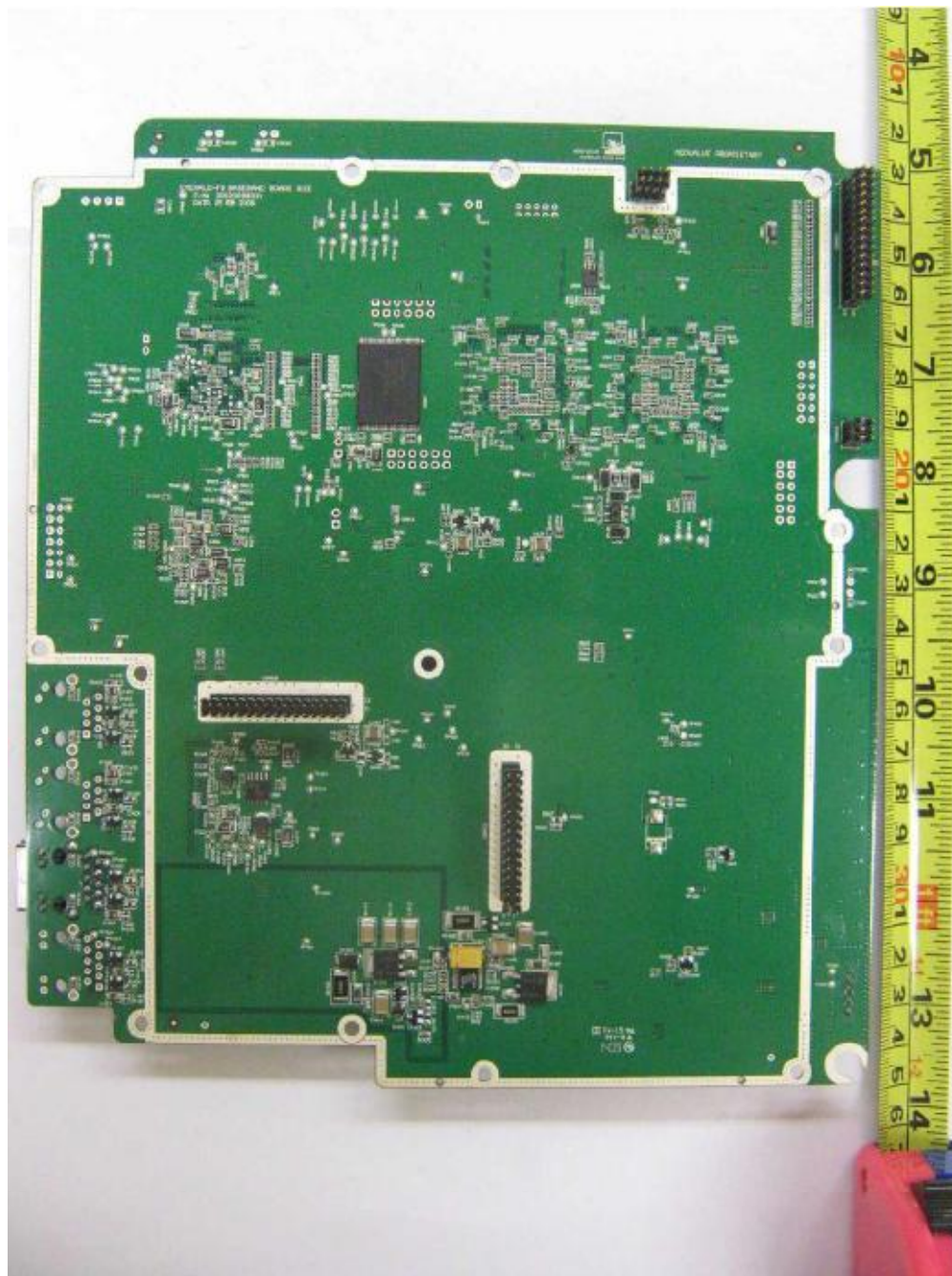
Base-Band Board PCB Trace Side
