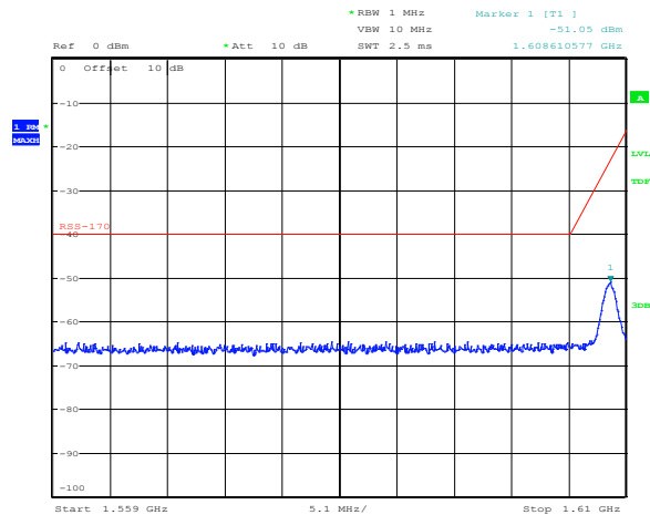
Figure 8.5-4: Emissions within 1559–1610 MHz, low channel, ISED limits
