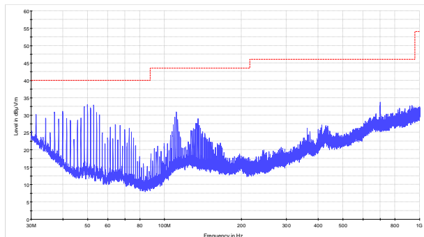
Figure 8.3-1: Spurious emissions below 1 GHz, low channel
